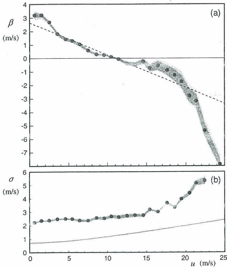
FIGURE 3 Like Figure 2 for the AVN winds.
