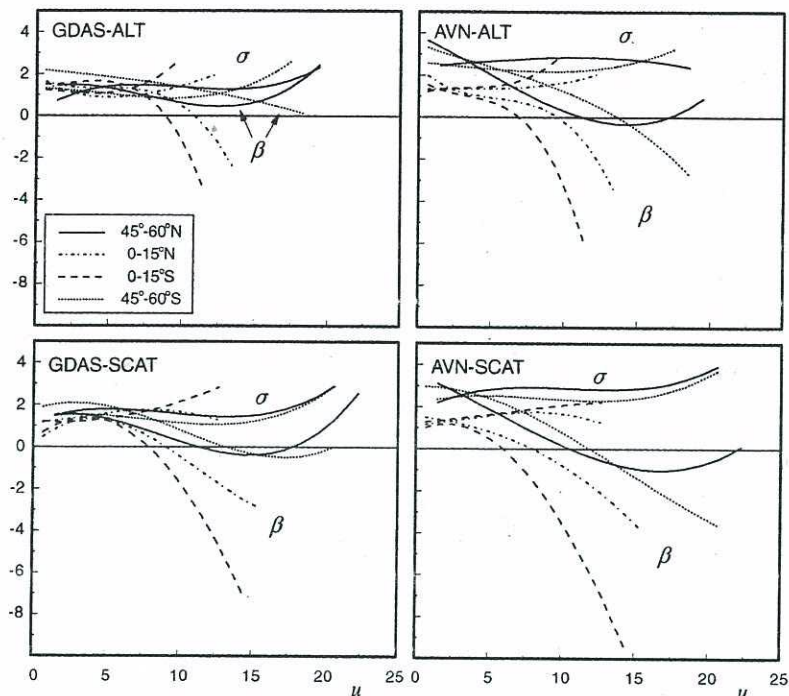
FIGURE 9 GDAS and AVN biases \beta and random errors (in \text{ms}^{-1} ) as a function of the observed wind speed u as estimated from ALT and SCAT data for four latitude bands. Biases and random errors represented by third-order polynomials. Note that \sigma is definite positive, whereas \beta has negative values in all except two lines in the upper left panel.
