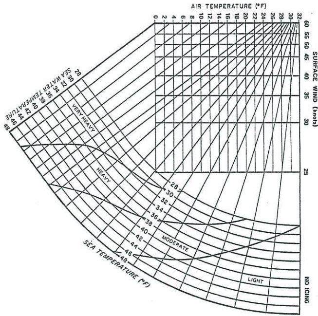
Fig. 1. Wise and Comisky (1980) Ice Accretion nomogram.
