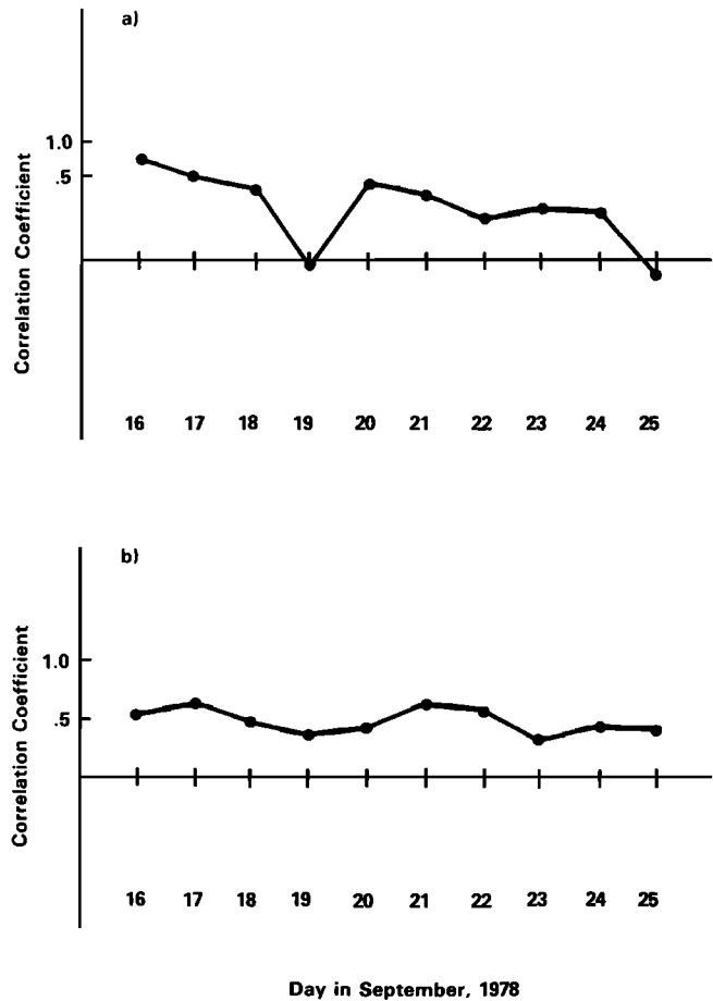
Fig. 8. Correlation coefficient between altimeter winds and NMC analysis for midnight (0000 UT) each day. (a) Northern hemisphere; (b) southern hemisphere.
