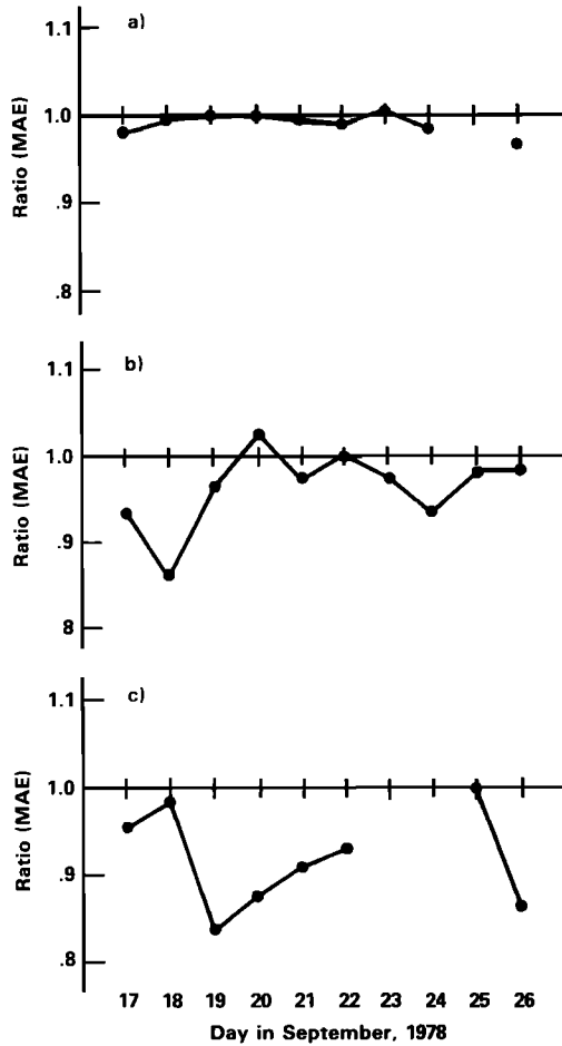
Fig. 7. Ratios of MAE for assimilation to control runs for SWH higher than 4 m. Latitudes are (a) between 30.0° and 62.5°N; (b) 62.5° and 30.0°S; and (c) 30.0°S and 0.0°. There were no SWH higher than 4 m for the northern equatorial belt.
