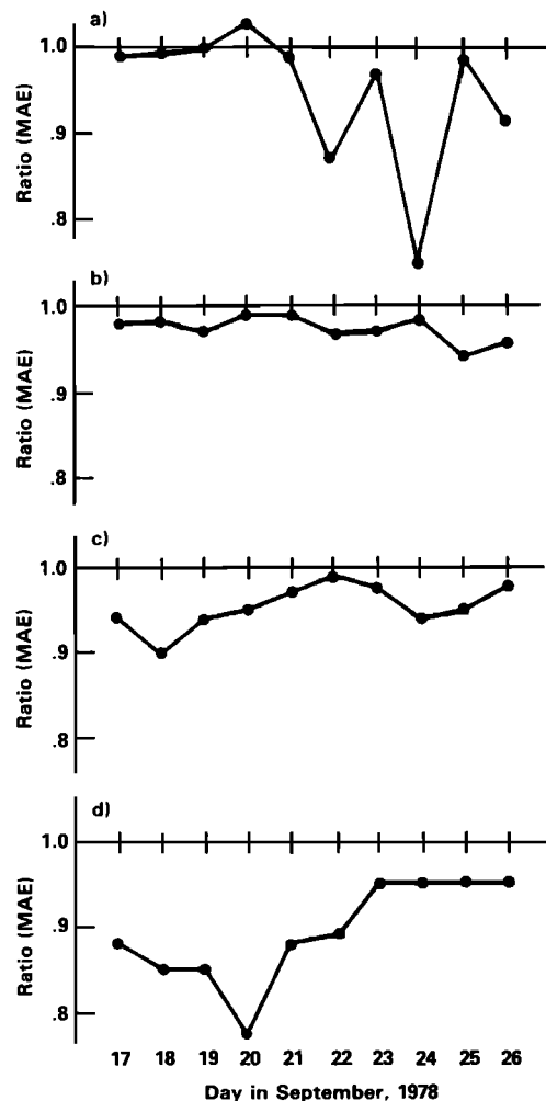
Fig. 6. Same as Figure 5, except for SWH higher than 2 m.
