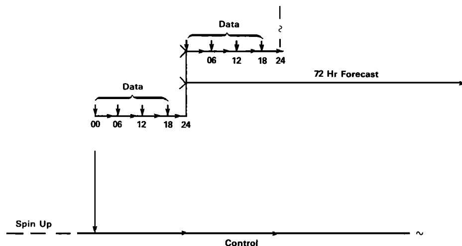
Fig. 1. Six-hour assimilation cycle. Vertical arrows indicate data insertion; horizontal arrows indicate forecast.
