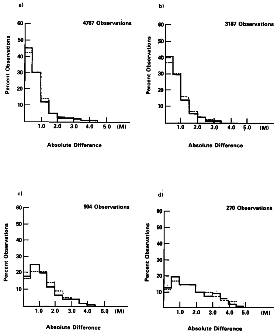
Fig. 4. Distribution of MAE for the control run (dashed curve) and for the assimilation run (solid curve), all forecasts, (a) for SWH higher than 0.5 m; (b) for SWH higher than 2 m; (c) for SWH higher than 4 m; (d) for SWH higher than 6 m.
