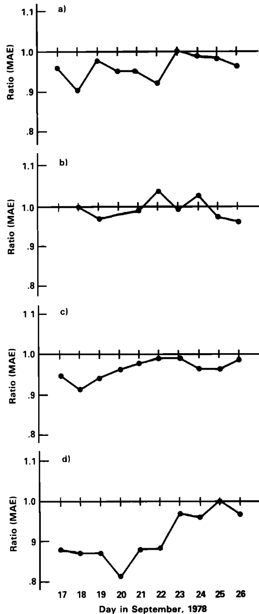
Fig. 5. Ratios of MAE for assimilation to control runs, for each day of the experiment, for SWH higher than 0.5 m. Latitudes are (a) between 0.0° and 30.0°N; (b) 30.0° and 62.5°N; (c) 62.5° and 30.0°S; and (d) 30.0°S and 0.0°
