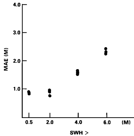
Fig. 3. MAE (in meters) for SWH grouped according to height for the control run: observed SWH higher than 0.5, 2, 4, and 6 m.
