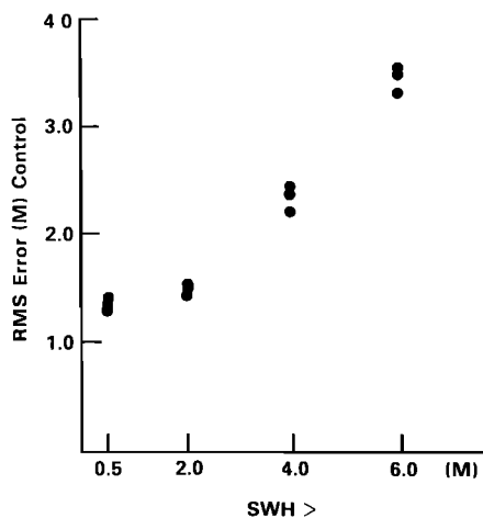
Fig. 2. The rms errors (in meters) for SWH grouped according to height for the control run: observed SWH higher than 0.5, 2, 4, and 6 m.
