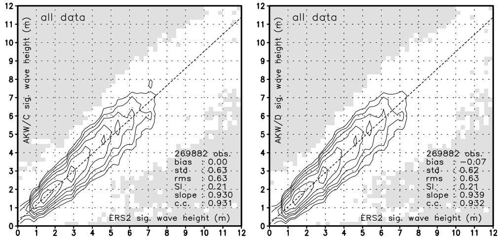
Fig. 5.12 : Like Fig. 5.11 for regional AKW model.
