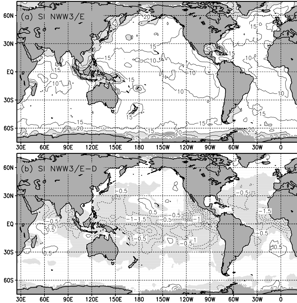
Fig. 6.1 : Scatter index (SI) in % of models against ERS-2 wave height data. Dark gray identifies lack of data. (a) NWW3/E model, contours at 5% intervals. (b) \Delta SI = NWW3/E - NWW3/D , contours at 0.5% intervals (note that contour levels are different from previous figures). Dotted contours correspond to negative values, \Delta SI = 0 contour not shown. Negative \Delta SI shaded light gray in black and white version.
