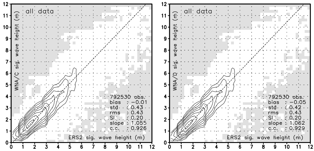
Fig. 5.13 : Like Fig. 5.13 for regional wna model.
