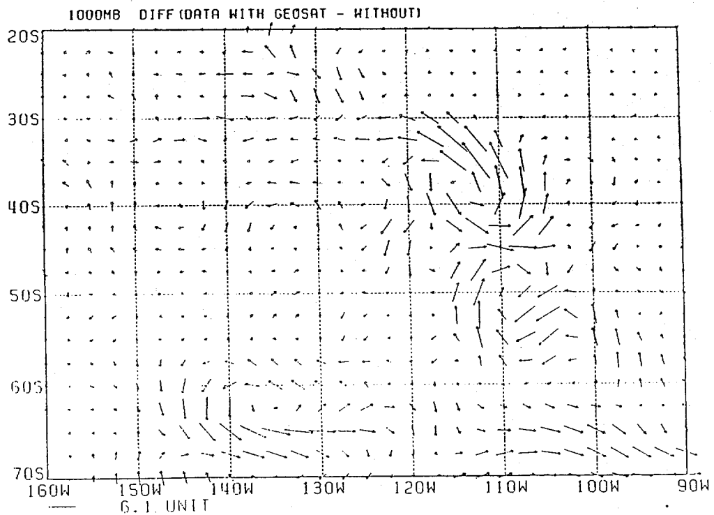
Figure 2: Same as Figure 1 except for the limited region enclosed between 90 W to 160 W longitude and 20 S to 70 S latitudes
