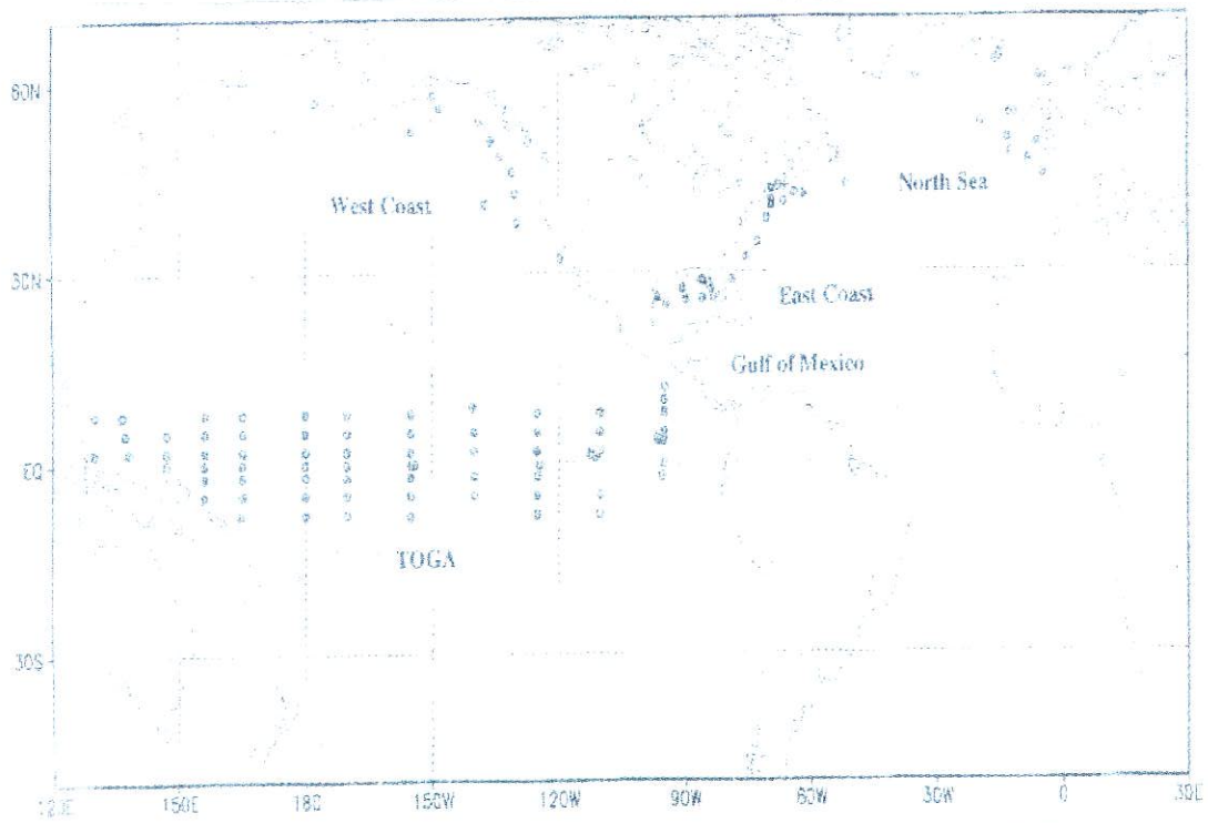
Figure 1. Distribution of deep water buoys for the five geographical regions: East Coast Atlantic Ocean, West Coast Pacific Ocean, North Sea, Gulf of Mexico, and TOGA regions.
