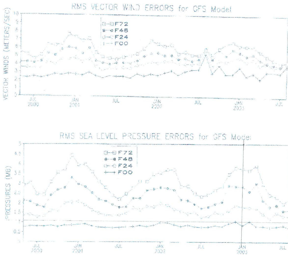
Figure 2. Time series of monthly mean RMS vector wind errors at 10 meters (top panel), and RMS sea level pressure errors (bottom panel) of the NCEP's operational GFS model. Forecasts for the period from May 2000 to August 2003.
