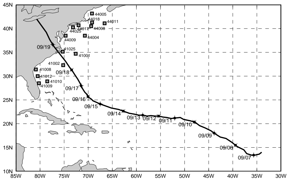
Fig. 2.1 : Buoy locations used in this study and the best guess track of hurricane Isabel. Dates along track correspond to 0000 UTC.
