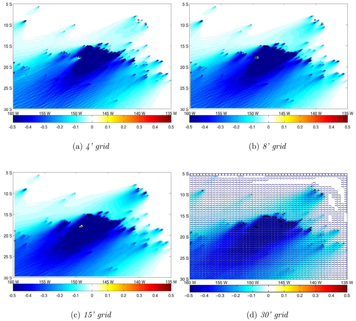
Fig. 3.23 : Differences between 2' and lower resolution grids (Test NO-OB)
