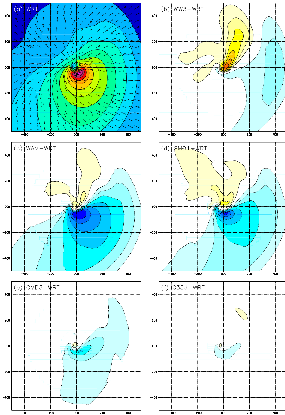
Fig. 5.2 : (a) Significant wave height H_s for the hurricane test test_hr and the WRT approach. Contour intervals at 1m and maximum wave height larger than 12m (b-f) Wave height difference in m for indicated approaches. Contour levels at 0.2m. Reds indicate positive difference. 0m difference contour not plotted.
