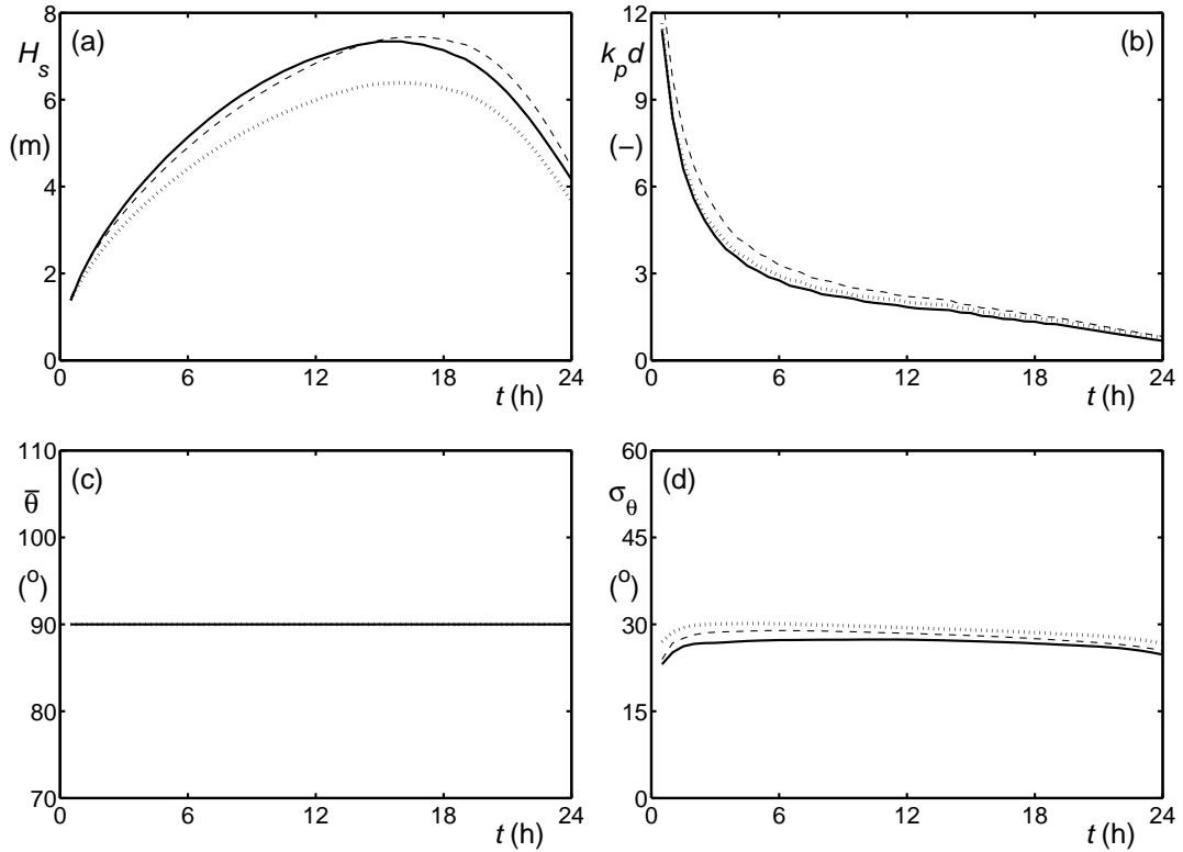
Fig. 3.21 : Evolution in time of a) significant wave height H_s , b) relative depth k_p d , c) mean direction \bar{\theta} , and d) directional spread \sigma_\theta for the depth- and time-limited growth test test_11. Solid line: WRT. Dashed line: WW3. Dotted line: WAM. Chain line: wind direction.
