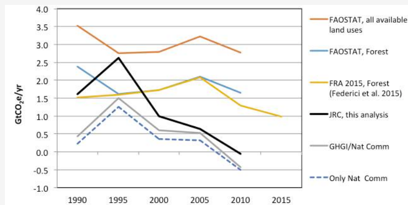
Figure 3. Different LULUCF-related historical datasets (at 5 years intervals; for FAO and NC data points represent 5-yrs averages). The JRC analysis in this report used the following source (in order of priority): INDCs; 2015 GHGIs; recent NCs (> 2010); other official country's documents; FRA 2015 (from Federici et al. 2015) complemented by FAOSTAT non-forest emissions. Note that, at the time of writing this report, net emissions from 'forest land' in FAOSTAT used FRA2010 data; this explains the differences with Federici et al. (2015), which is based on FRA 2015. See http://faostat3.fao.org/download/G2/*/*E for methodologies used by FAOSTAT.
