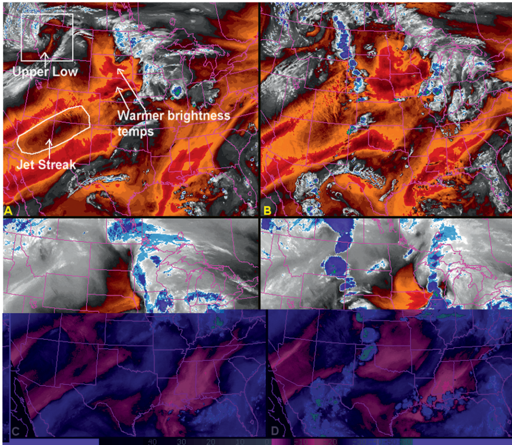
FIG. 1. NSSL 4-km WRF-ARW synthetic satellite imagery for the 6.95\text{-}\mu\text{m} (water vapor) band from the 0000 UTC 21 Jun 2010 model run valid at (a) 1700 and (b) 0100 UTC 22 Jun. GOES-13 imagery for the 6.5\text{-}\mu\text{m} (water vapor) band at (c) 1703 and (d) 0102 UTC 22 Jun. The brightness temperature scale ( ^{\circ}\text{C} ) is the same for the synthetic and GOES imagery. Animated loops between 1200 and 0100 UTC are also available for the synthetic imagery along with overlays for 250- and 500-hPa geopotential heights (m), along with 250-hPa isotachs ( \text{m s}^{-1} ) ( http://rammb.cira.colostate.edu/redirect/21jun10_synth_band9 ) and the GOES imagery ( http://rammb.cira.colostate.edu/redirect/21jun10_goes_wv ).
