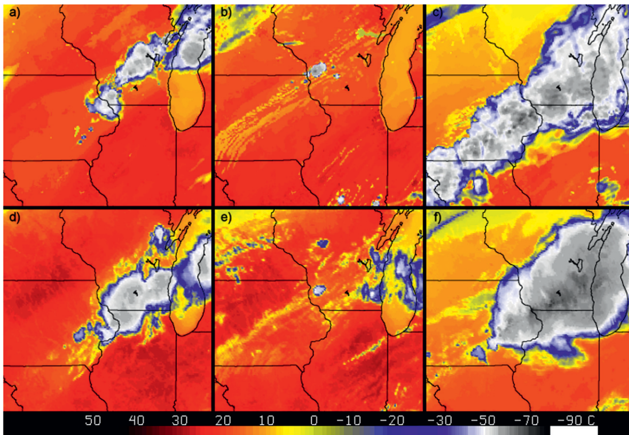
FIG. 6. NSSL 4-km WRF-ARW synthetic imagery for the 11.2- \mu\text{m} (IR) band from the 0000 UTC 8 Jun 2011 model run valid at (a) 1500 UTC 8 Jun, (b) 2100 UTC 8 Jun, and (c) 0200 UTC 9 Jun 2011. GOES-13 imagery for the 10.7- \mu\text{m} (IR) band at (d) 1515 UTC 8 Jun, (e) 2132 UTC 8 Jun, and (f) 0202 UTC 9 Jun 2011. The brightness temperature scale ( ^{\circ}\text{C} ) is the same for the synthetic and GOES-13 imagery. Animated loops between 1400 UTC 8 Jun and 0300 UTC 9 Jun 2011 are also available for the synthetic imagery ( http://cimss.ssec.wisc.edu/goes_r/proving-ground/nssl_abi/08june2011/08june2011_abi_ir.html ) and the GOES imagery ( http://cimss.ssec.wisc.edu/goes_r/proving-ground/nssl_abi/08june2011/08june2011_goes_ir.html ).
