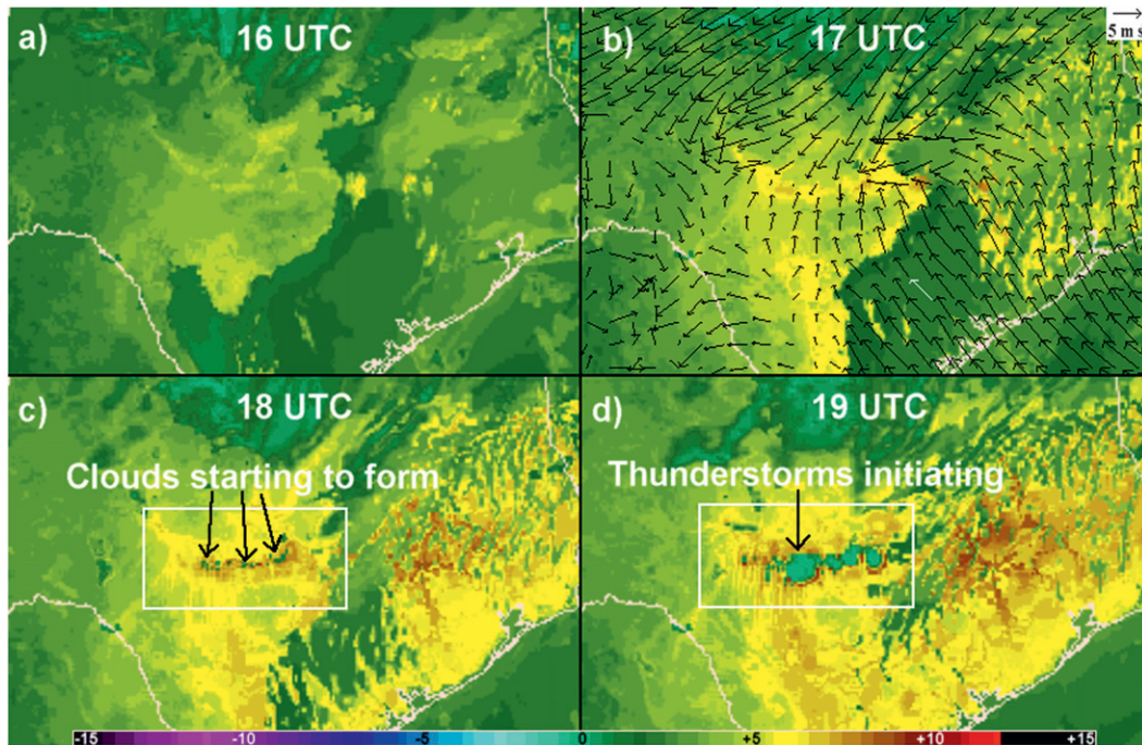
FIG. 7. Synthetic 10.35–12.3- \mu\text{m} band from the NSSL WRF 0000 UTC 20 Apr 2011 (a) 16-, (b) 17-, (c) 18-, and (d) 19-h forecasts. The brightness temperature difference scale in ^{\circ}\text{C} . Warmer colors represent more positive values. The images appear as they do in N-AWIPS, the operational display software at the SPC. The vectors in (b) are the 10-m winds from the NSSL WRF and the green areas within the boxes in (c) and (d) are convective clouds.
