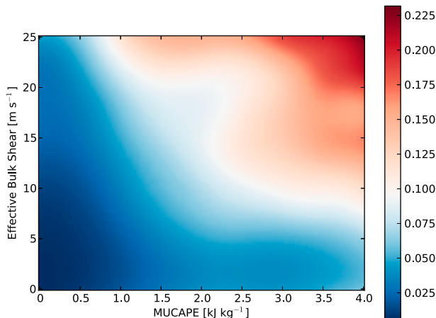
FIG. 2. Table of a priori probability of severe for identified storms, given their median effective bulk shear and median MUCAPE.
