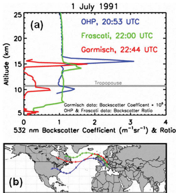
FIG. 5. Three European aerosol lidar profiles on 1 Jul 1991, and back trajectories. Locations are Garmisch-Partenkirchen, Germany (47.5°N, 11.1°E); Haute Provence Observatory (OHP), France (44.0°N, 6.0°E); and Frascati, Italy (41.8°N, 12.7°E). (a) Garmisch data are 532-nm backscatter coefficient ( m^{-1} sr^{-1} ) scaled by 10^6 . Frascati and OHP data are 532-nm backscatter ratio, that is, (aerosol + Rayleigh)/Rayleigh. Tropopause height averaged from radiosonde profiles nearest the lidars. (b) Isentropic back trajectories from LS aerosol layers beginning at 2200 UTC 1 Jul and ending at 2200 UTC 20 Jun. Dots at 0000 UTC. Trajectory model described by Schoeberl and Sparling (1995). Credit for data access: NASA Goddard Automailer.
