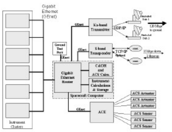
Figure 6.5: SDO CD&H system.
