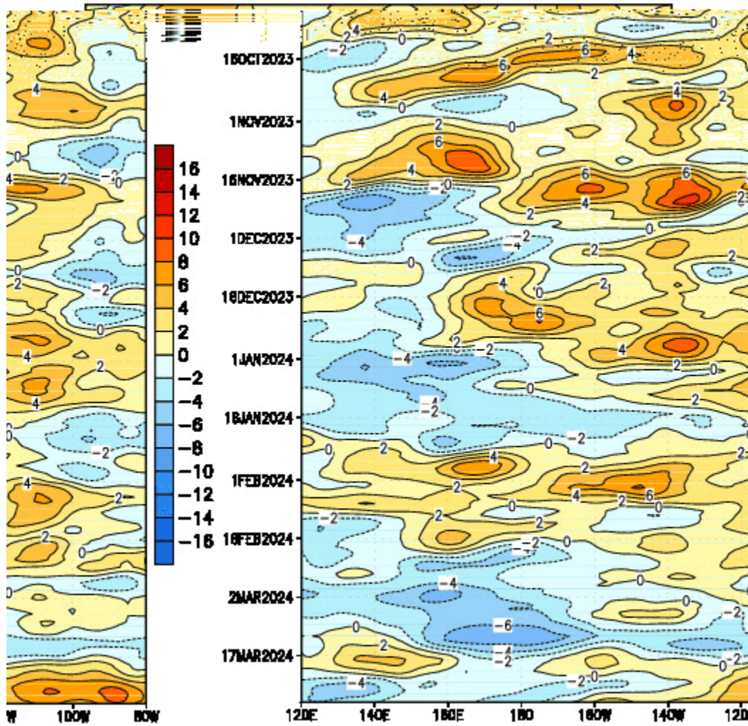
Figure 22: Anomalous equatorial low-level winds spanning from 120°E to 80°W. Figure courtesy of Climate Prediction Center.
