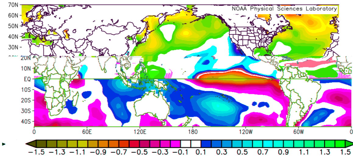
Figure 12: Average August–October SST anomalies in our seven analog years.
