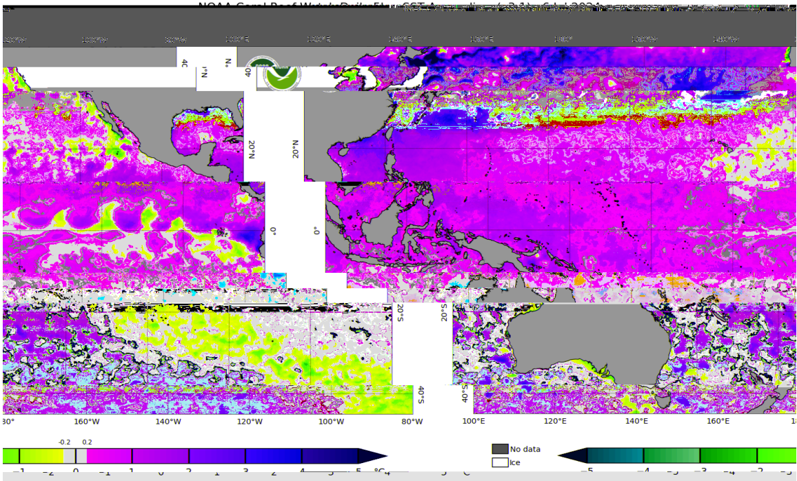
Figure 21: Current SST anomalies across the tropical and subtropical Pacific.
