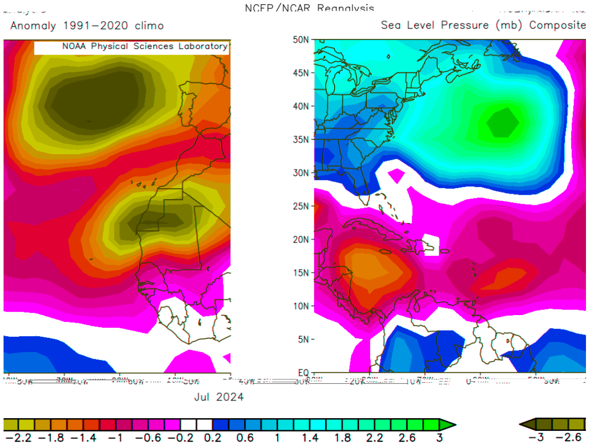
Figure 30: July-averaged sea level pressure anomalies in 2024 across the tropical and subtropical North Atlantic.
