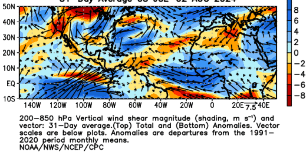
Figure 28: 3 July – 2 August-averaged vertical wind shear across the tropical and subtropical Atlantic differenced from the 1991–2020 climatology.
