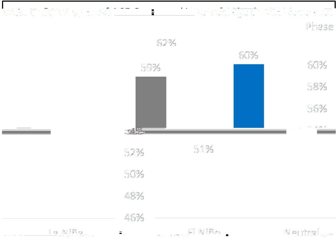
Figure 16: Percentage of ACE generated west of 60°W by ENSO phase.
