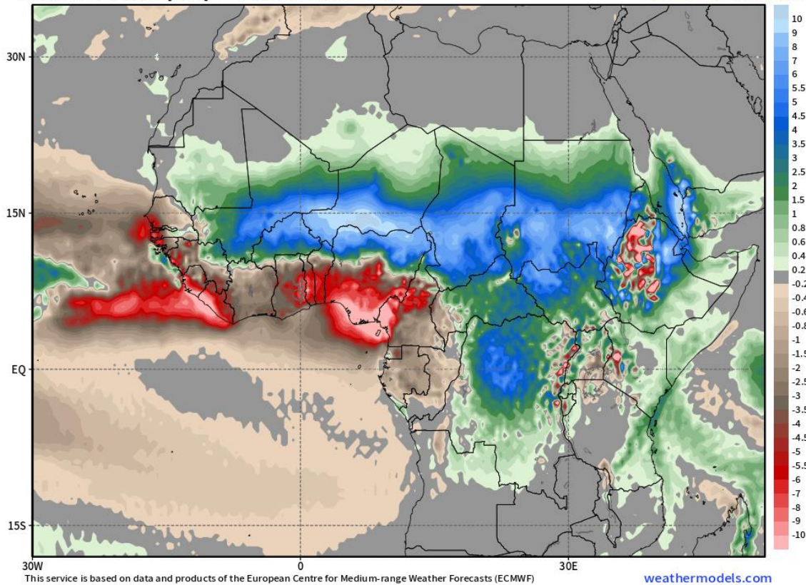
Figure 35: Forecast precipitation across North Africa through 15 September from the ECMWF ensemble.
