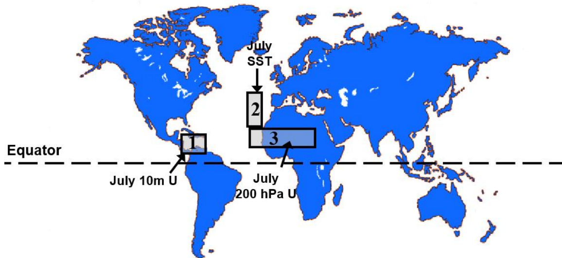
Figure 1: Location of predictors for the post-31 July forecast for the 2024 hurricane season from the July-averaged statistical model.
