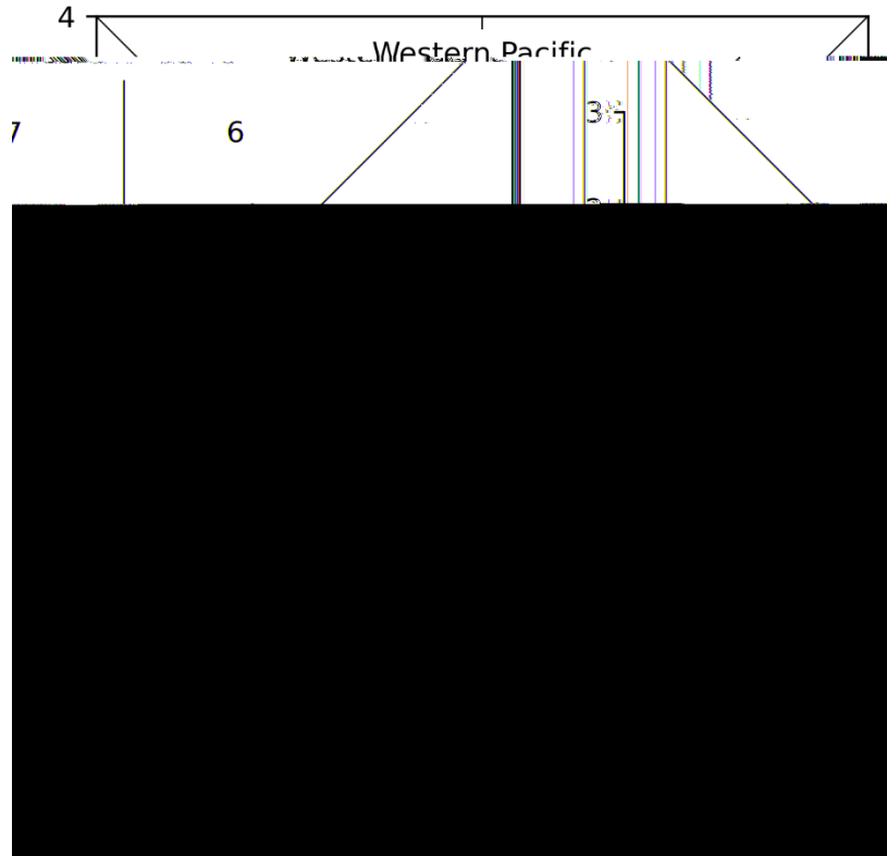
Figure 2: Propagation of the Madden-Julian Oscillation (MJO) based on the Wheeler-Hendon classification scheme over the period from 1 August to 19 November. The Maritime Continent refers to Indonesia and the surrounding islands. RMM stands for Real-Time Multivariate MJO. Figure courtesy of Carl Schreck.
