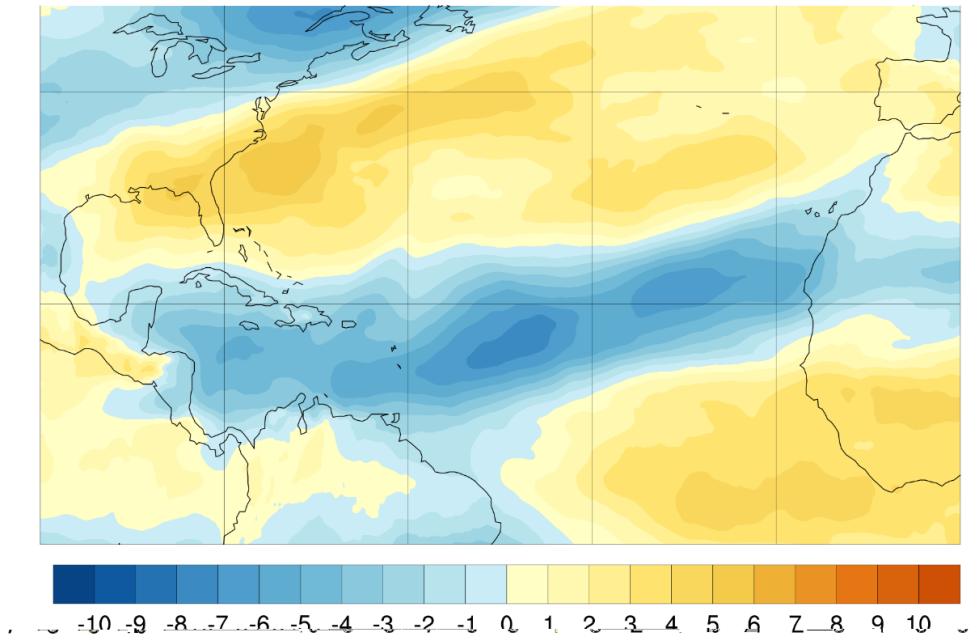
Figure 12: Anomalous North Atlantic vertical wind shear ( \text{m s}^{-1} ) from August–October 2024.
