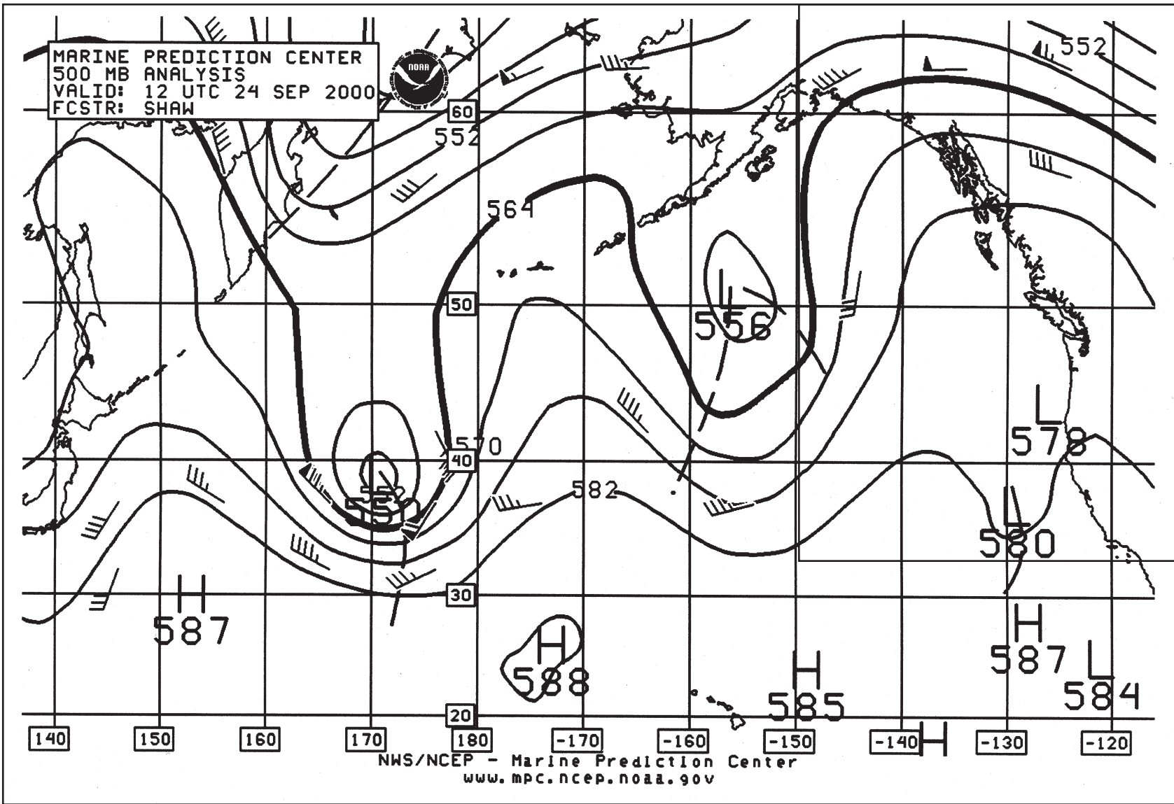
Figure 2. MPC 500-Mb Analysis of North Pacific valid at 1200 UTC September 24, 2000.
