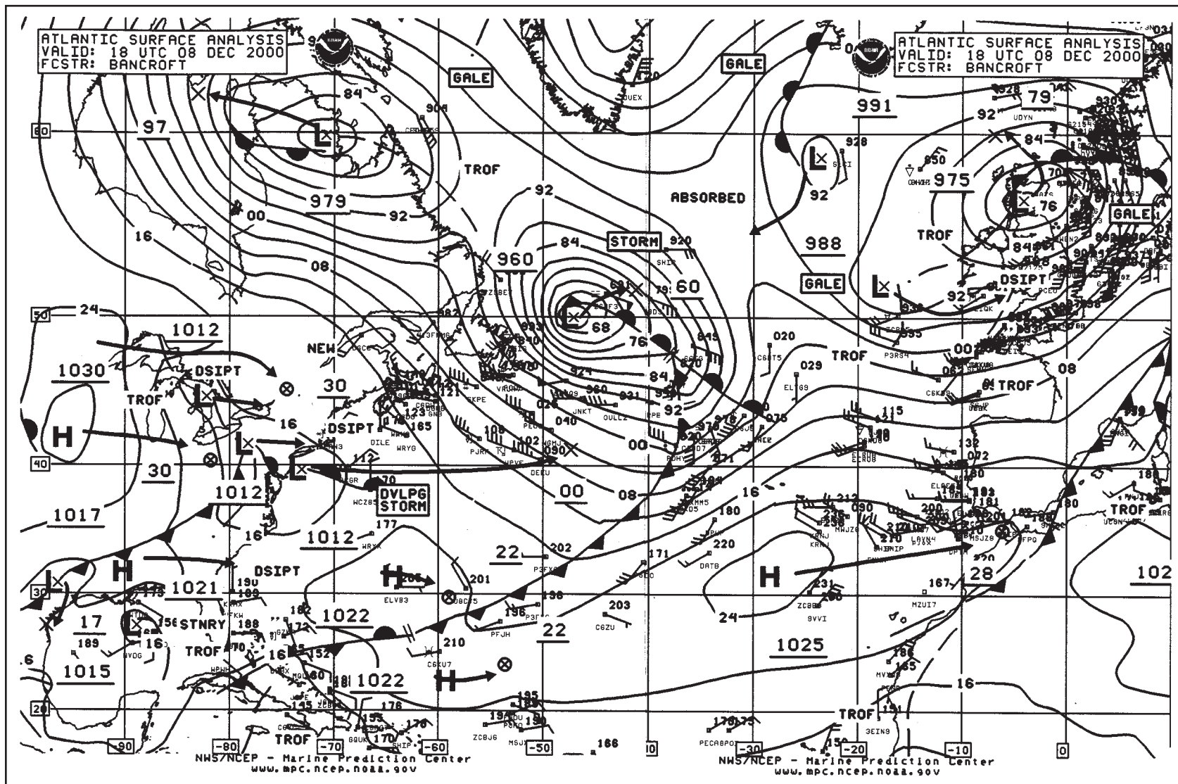
Figure 13. MPC North Atlantic Surface Analysis chart valid at 1800 UTC December 8, 2000.
