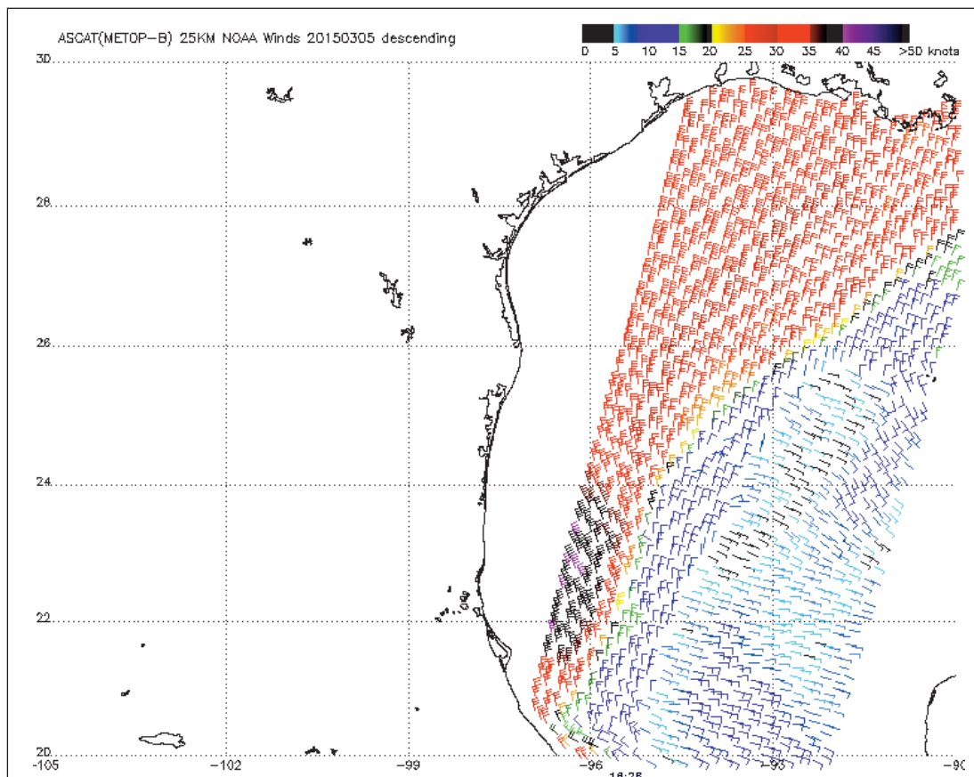
Figure 3. A scatterometer pass from the MetOp Advanced SCATERometer (ASCAT-B) valid around 1628 UTC 05 March. Note the brown and pink wind barbs in the southwestern Gulf of Mexico indicating gale to storm force winds.
