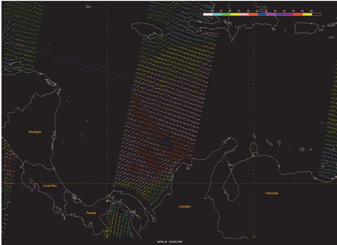
Figure 2. A scatterometer pass from the MetOp Advanced SCATerometer (ASCAT-B) valid around 1508 UTC 05 January. Note the dark blue wind barbs in the Southwestern Caribbean Sea indicating gale force winds between 34 and 40 kts.
