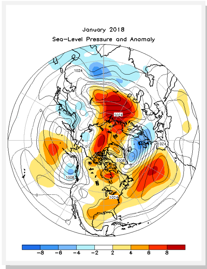
Figure 2. Northern Hemisphere mean and anomalous sea level pressure (CDAS/ Reanalysis). Mean values are denoted by solid contours drawn at an interval of 4 hPa. Anomaly contour interval is indicated by shading. Anomalies are calculated as departures from the 1981–2010 base-period monthly means.
