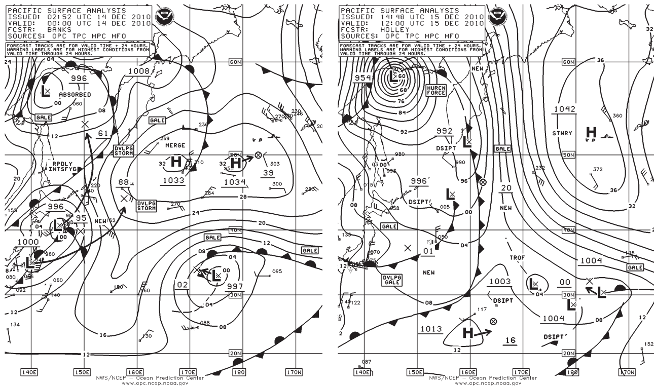
Figure 19. OPC North Pacific Surface Analysis charts valid 0000 UTC December 14 and 1200 UTC December 15, 2010.
