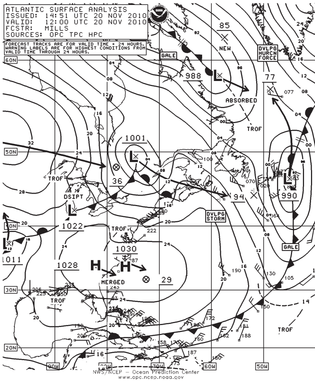
Figure 14. OPC North Atlantic Surface Analysis charts valid 1200 UTC November 20 and 21, 2010.
