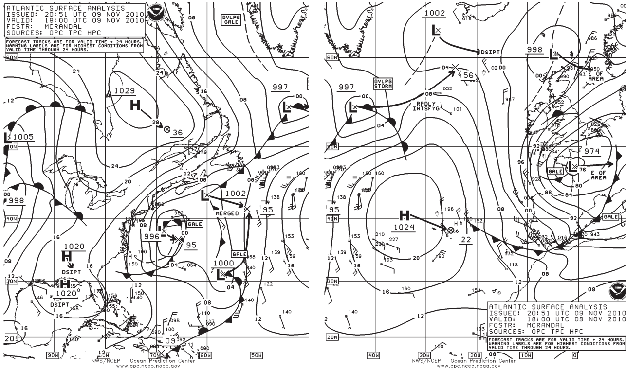
Figure 11. OPC North Atlantic Surface Analysis charts valid 1800 UTC November 9, 2010.
