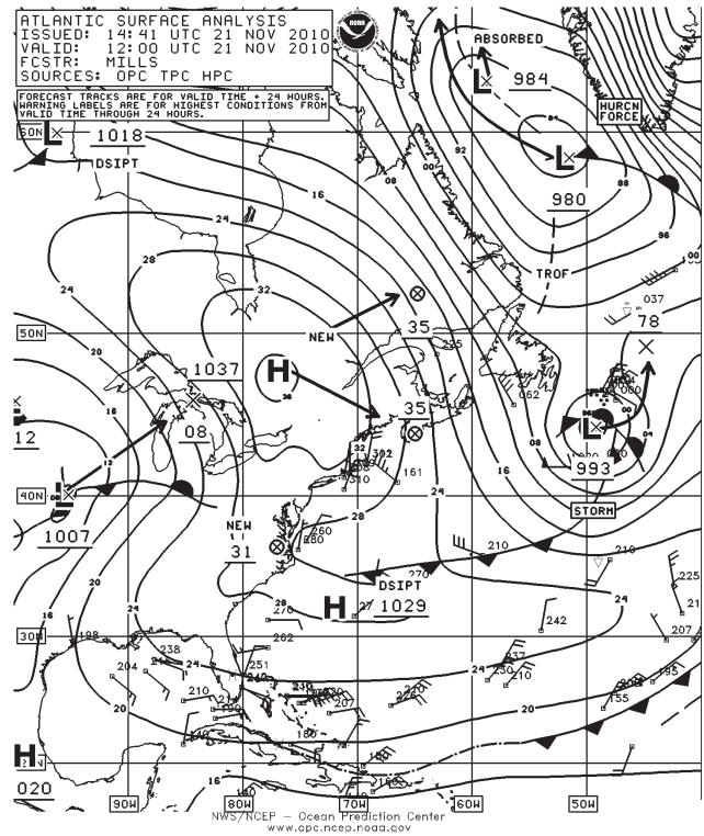
Figure 14. OPC North Atlantic Surface Analysis charts valid 1200 UTC November 20 and 21, 2010.
