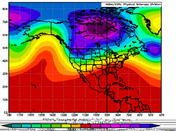
Mean geopotential 500mb heights for 11/22/10 to 11/24/10
