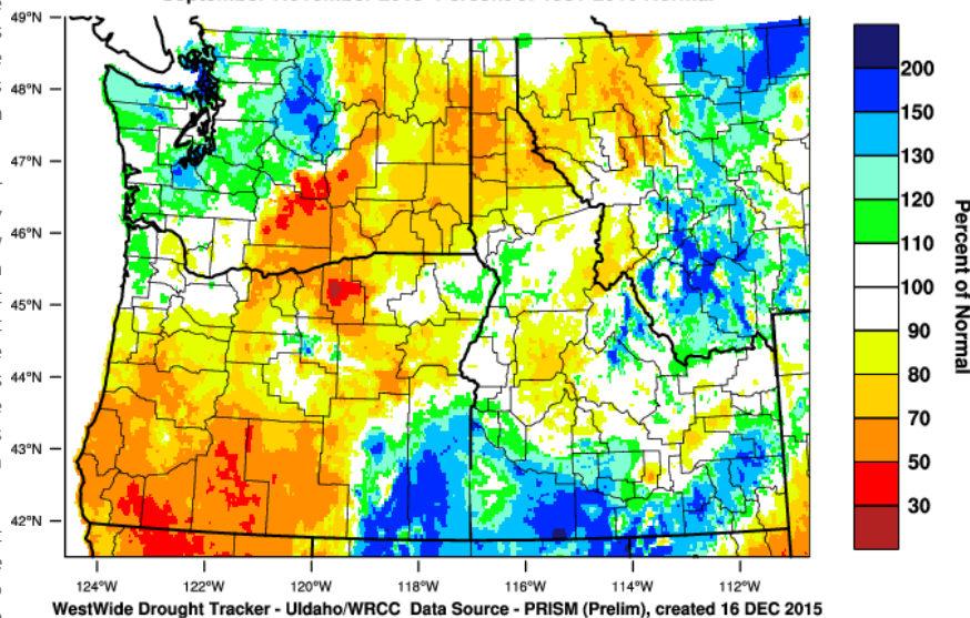
September-November 2015 Percent of 1981-2010 Normal
