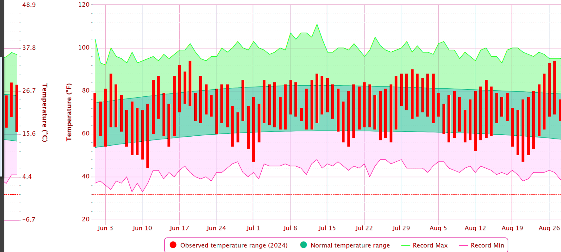
Daily Temperature Data – Saginaw Area, MI (ThreadEx)
