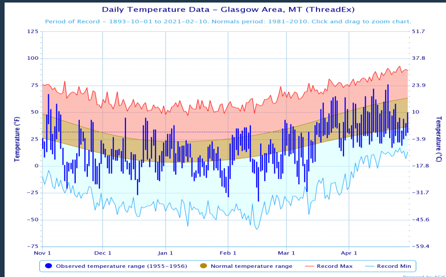
Figure 2: Glasgow, MT climate graphs from November 29, 1955 to April 21, 1956.
