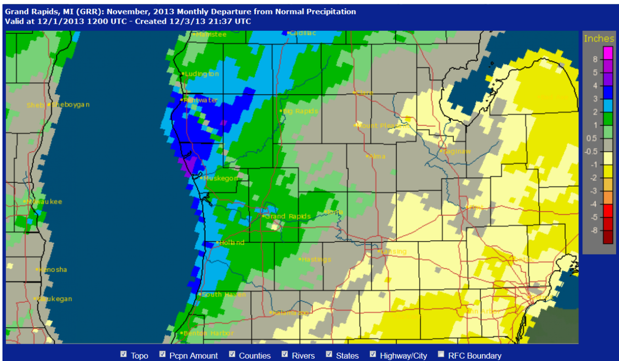
Figure 2. November Monthly Departure from Normal Precipitation Totals
