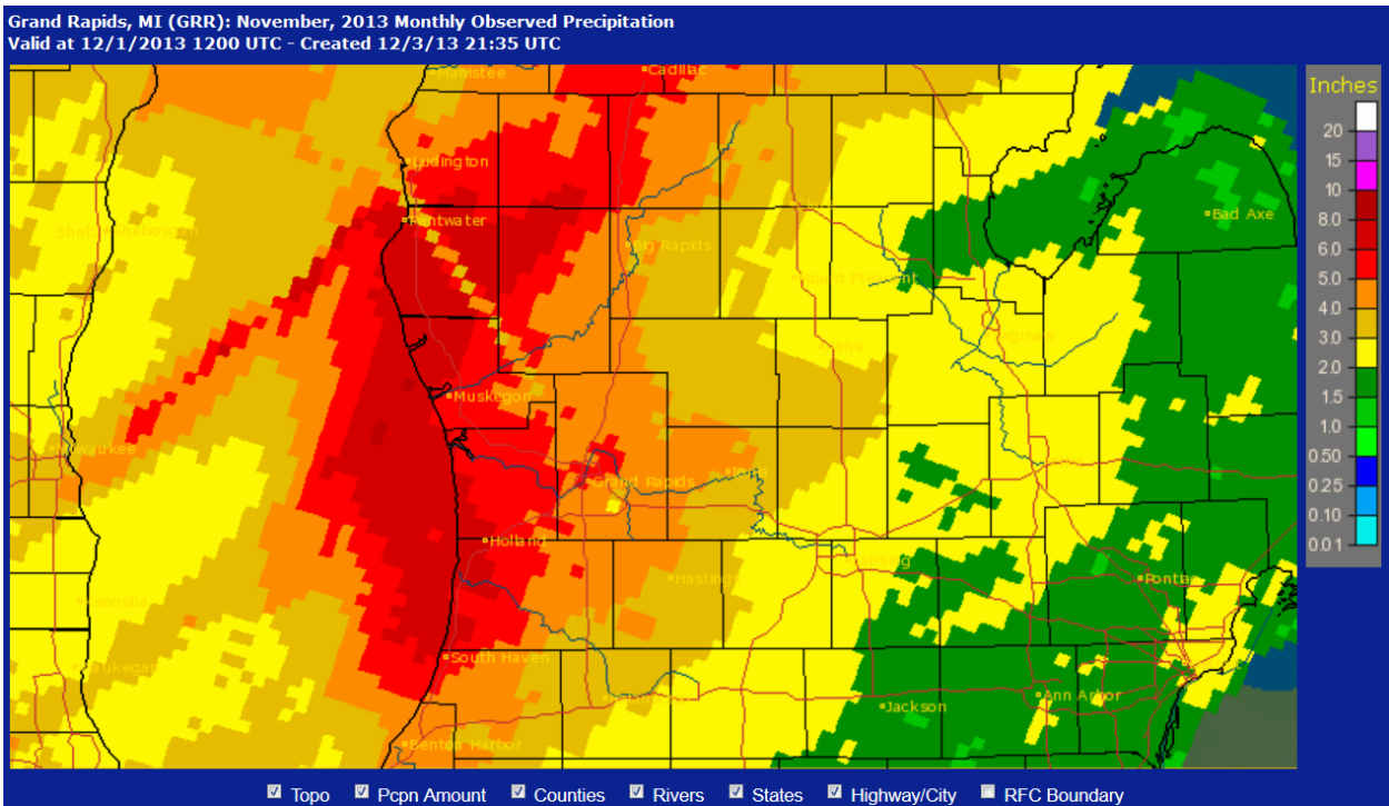
Figure 1. November Monthly Precipitation Totals
