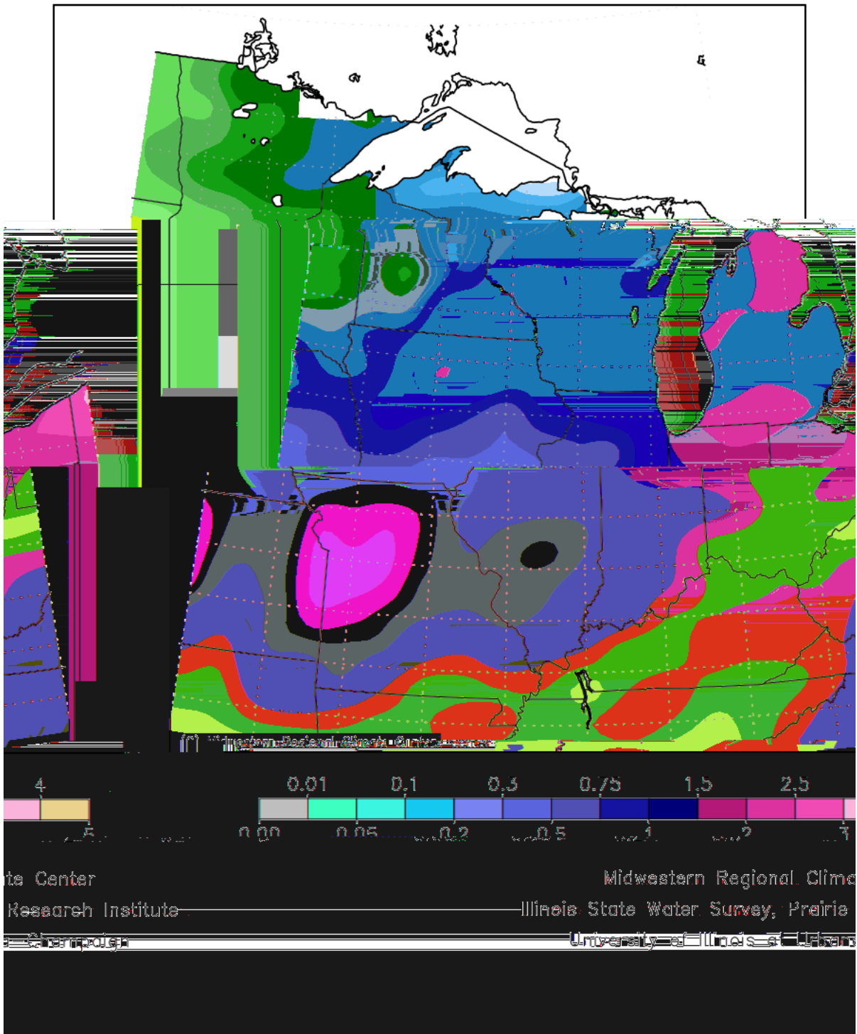
Figure 1. February Monthly Precipitation Totals
