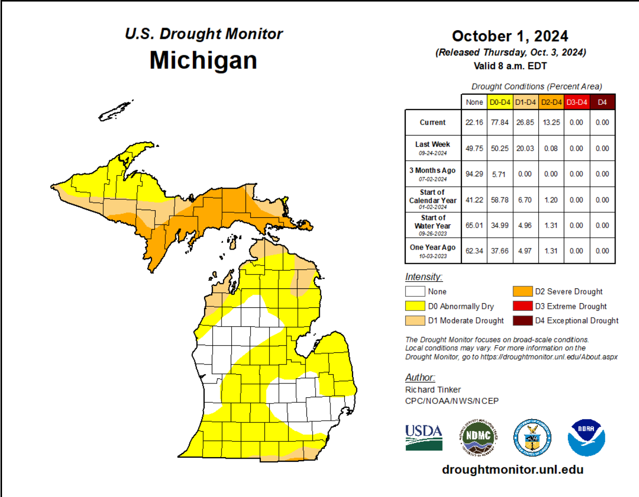
Figure 5.U.S. Drought Monitor effectively shows an expanding drought across the lower peninsula.
