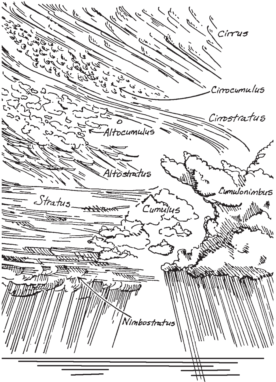
Cloud types.
