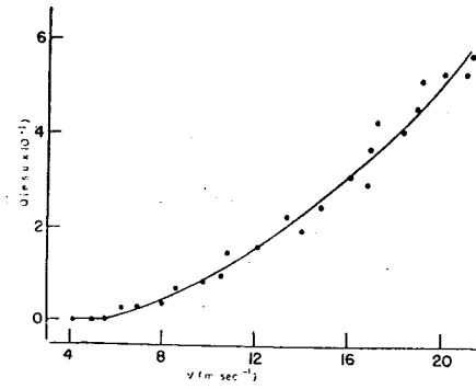
Fig. 2. The charge Q acquired by a smooth ice sphere exposed to a stream of snow crystals as a function of the velocity of impact V
