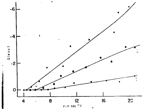
Fig. 3. The charge Q acquired by ice spheres of irregular surface structure exposed to a stream of snow crystals as a function of the velocity of impact V : (1) exceedingly irregular, (2) very irregular, (3) irregular surface structure
