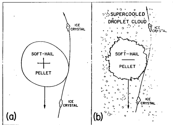
Fig. 4. Asymmetric rubbing with ice crystals confers (a) positive, (b) negative charge on a soft-hail pellet, according to its surface structure
