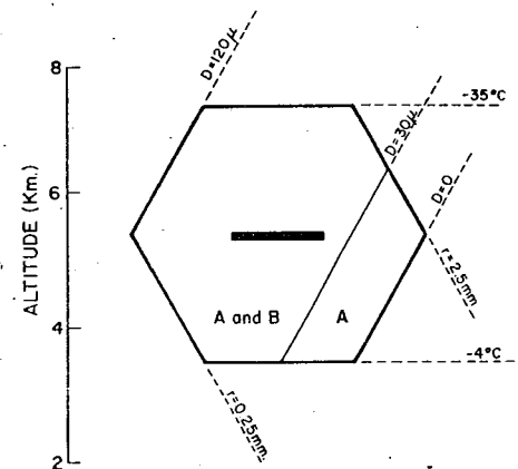
Fig. 5. The ranges of pellet radius r , supercooled droplet diameter D , and temperature T over which a growing pellet of soft hail acquires appreciable negative charge by means of (A) ice-crystal-hailstone collisions and (B) supercooled droplet shattering
