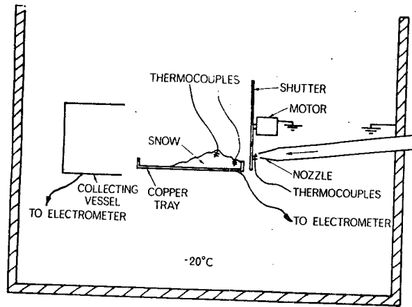
Fig. 1. Apparatus for measuring the electrification produced when snow is disrupted by an air jet
