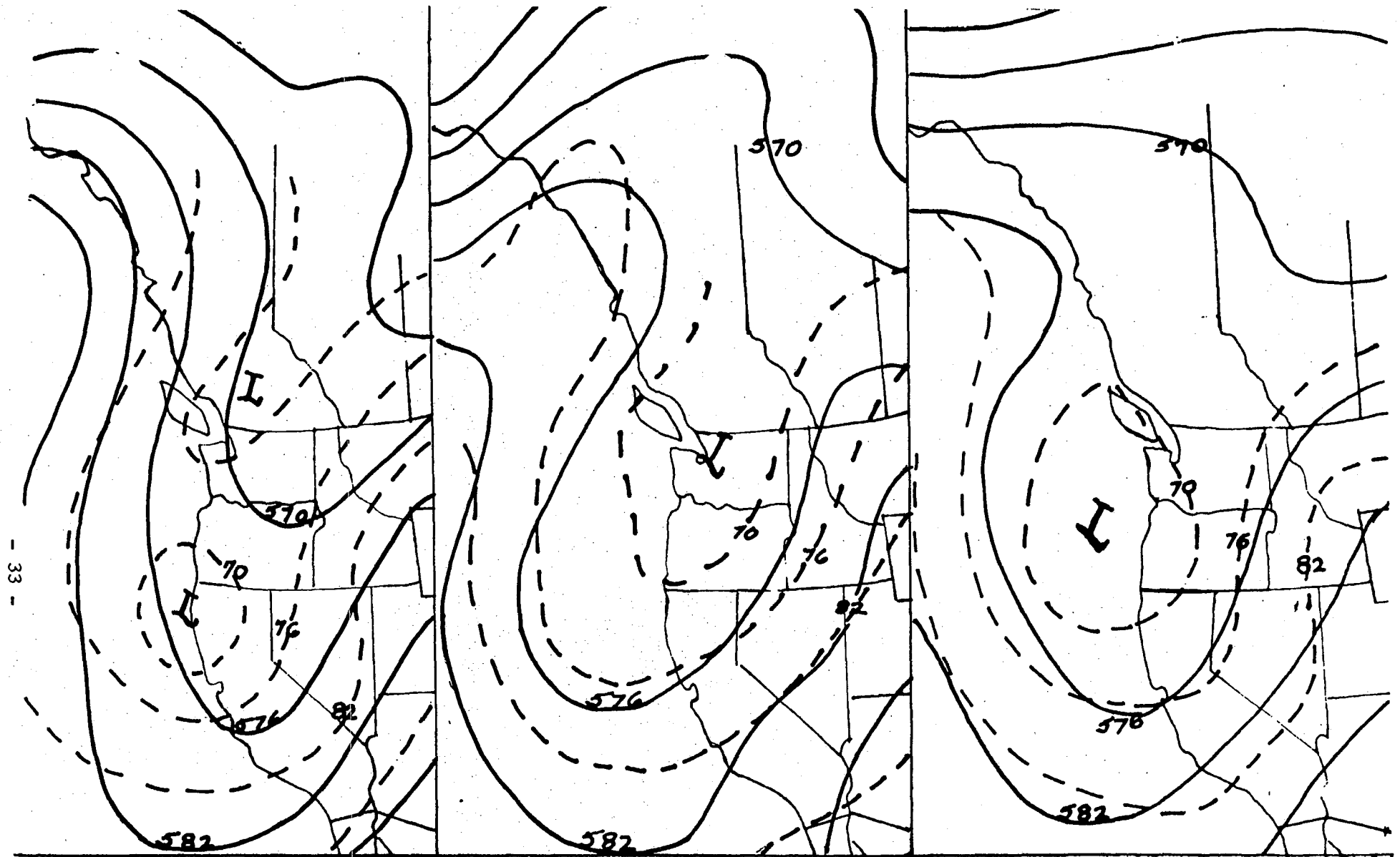
FIGURE 2a. 3-LEVEL 36-HOUR 500-MB PROGNOSIS, VALID 1200Z JULY 12, 1966. Solid lines are prognostic contours; dashed lines, verifying contours. Both sets of contours are labeled in decimeters, the 5 being omitted from verifying contours. Initial analysis for forecast is given in Figure 1.
