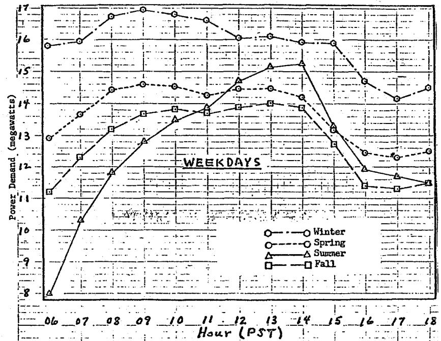
Figure 5. Nevada Test Site power demand during weekday daytime hours, by season.
