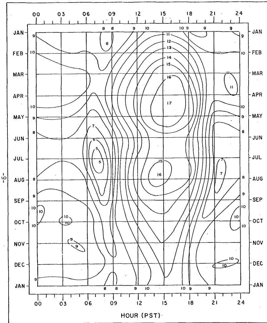
Figure 2. Average wind speed in miles per hour as a function of time of day. Station: BJJ
