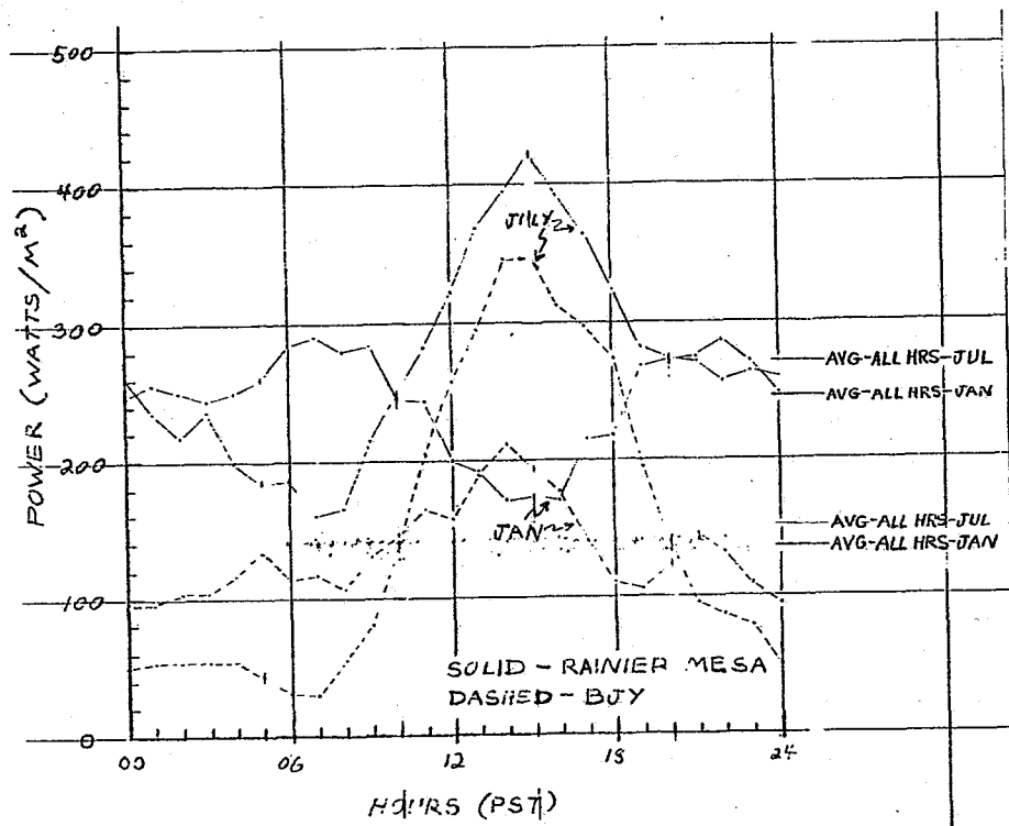
Figure 4. The diurnal average wind power availability profile for NTS stations, BJJ and Rainier Mesa, for July and January, with daily average wind power for each curve indicated.
