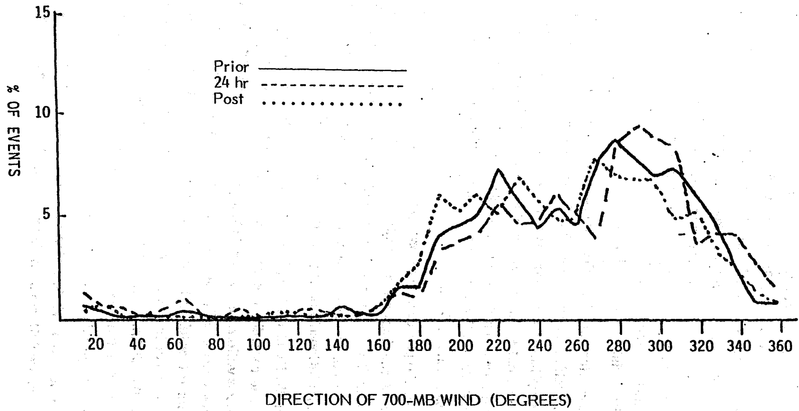
Figure 2. The percentage of all precipitation events at Alta is plotted three ways with respect to the 700-mb wind direction at 00Z. One line is from checking only intensity observations prior to 00Z. A second line is checking only observations after (post) 00Z. The third line is based on the 24 hour precipitation measurement taken at 8am.
