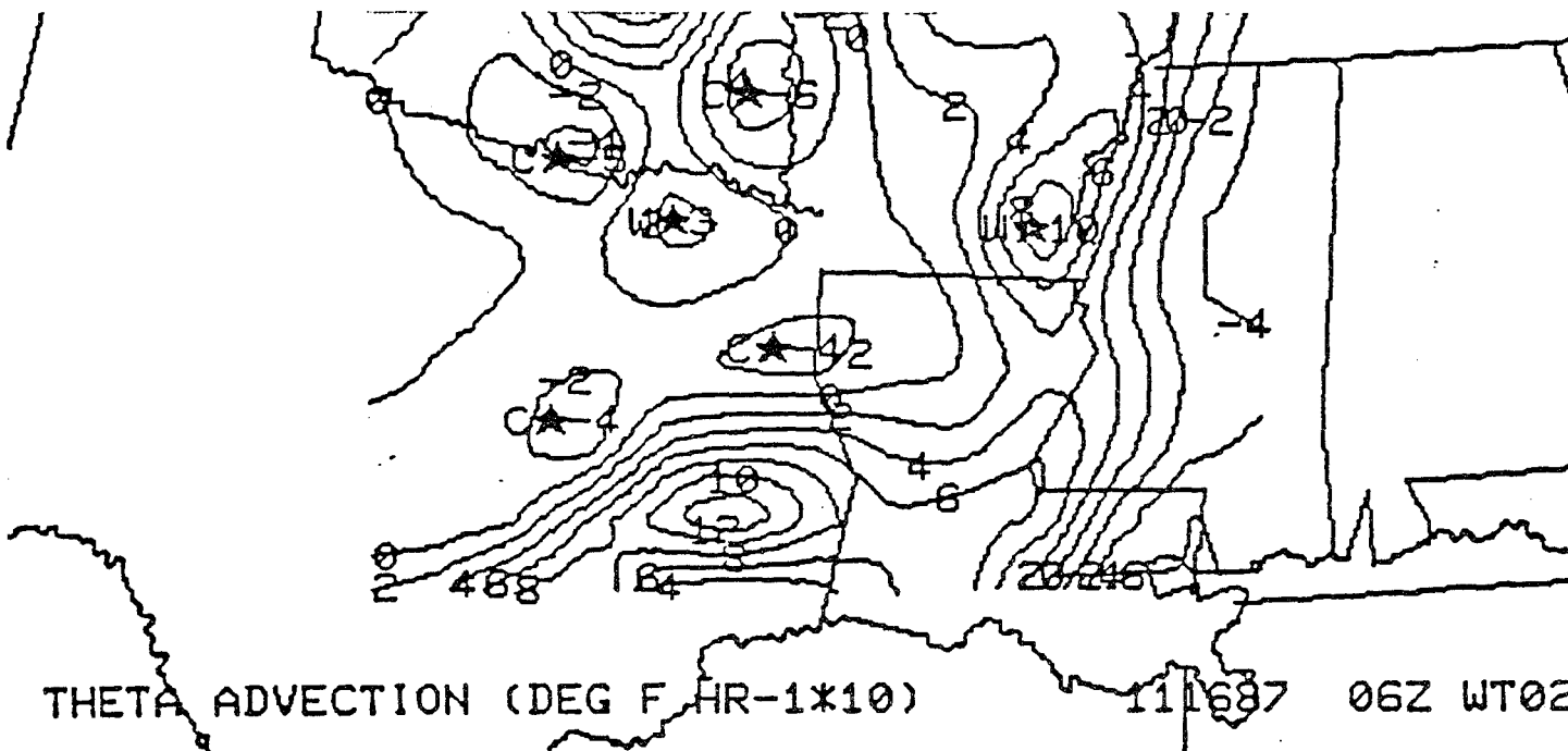
Fig. 14a Theta advection. 06Z November 16, 1987.
