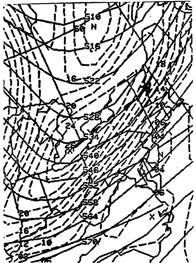
Figure 10. Initial NGM 500 mb Heights and Vorticity
