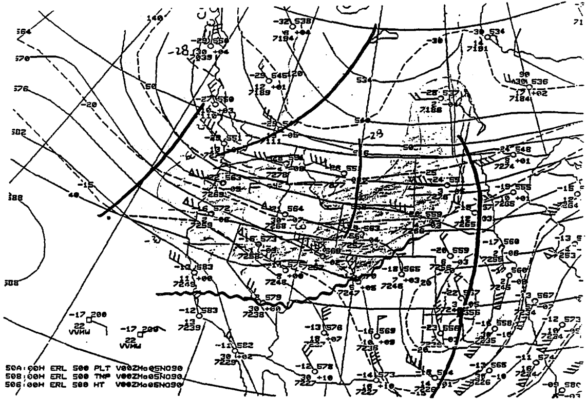
Figure 3a. 500 mb (50Kpa) constant pressure analysis for 05 Nov 1990, 00 UTC. Solid lines are intervals of 60 geo-potential meters. Dashed lines are intervals of 5 deg. C. Shading indicates areas of dew point depression 5 deg. C. or less.
