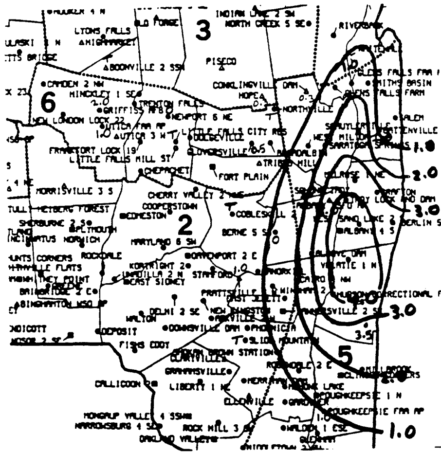
Figure 14. Mesoscale snowburst event total snowfall (inches), for 1200 UTC, February 25, 1990 thru 0000 UTC, February 26, 1990.
