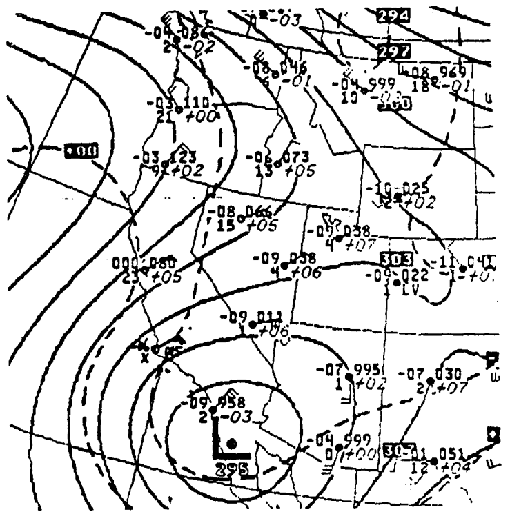
Figure 44b. 0000 UTC 15 November 1993 700mb analysis heights/temperature
