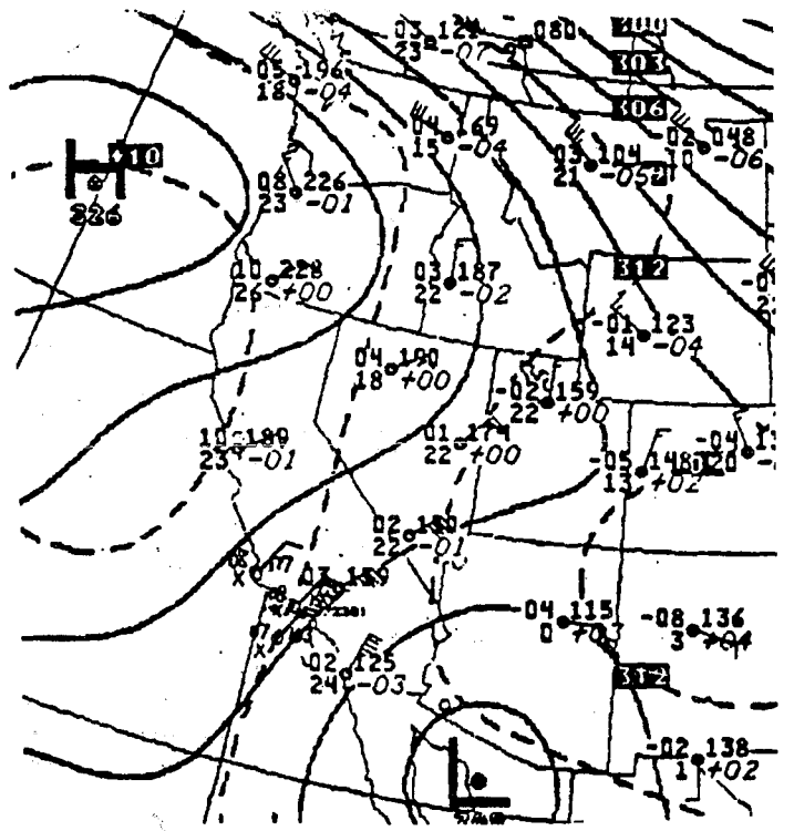
Figure 6b. 1200 UTC 27 October 1993 700mb analysis heights/temperature
