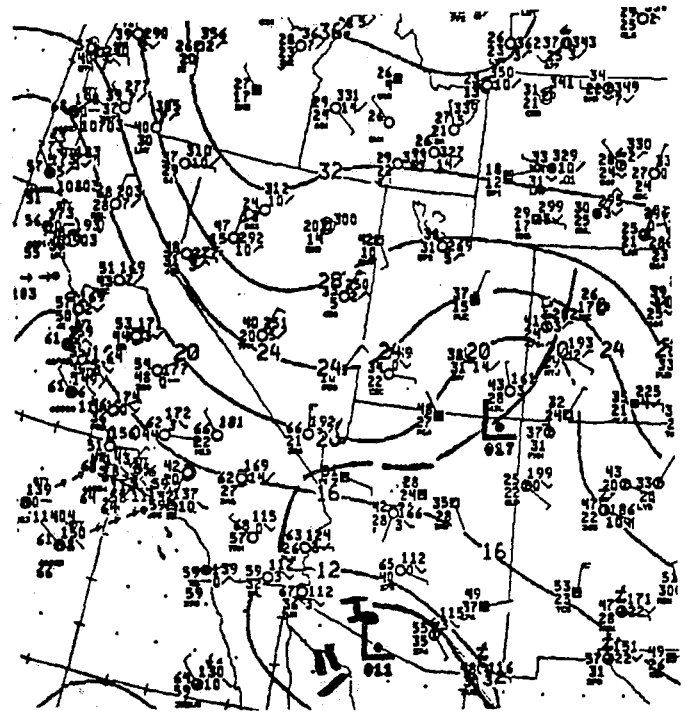
Figure 5b. 1200 UTC 26 October 1993 NMC surface analysis
