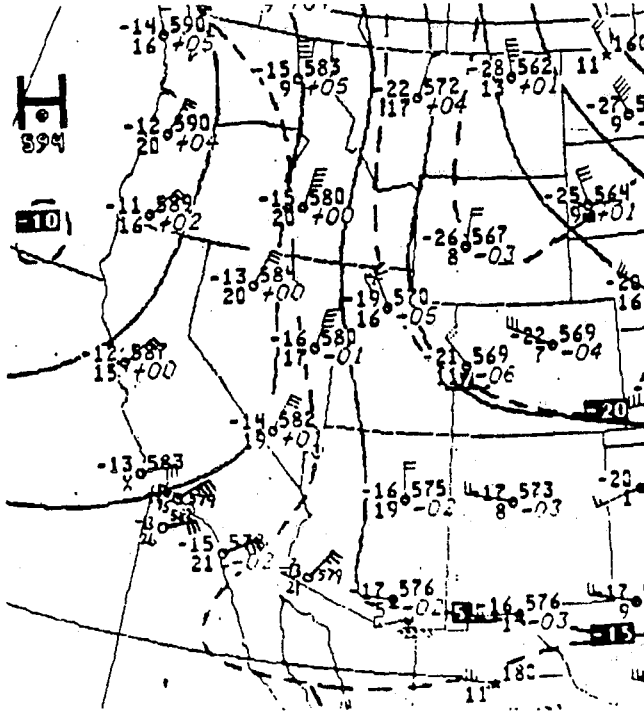
Figure 5a. 1200 UTC 26 October 1993 500mb analysis heights/temperature
