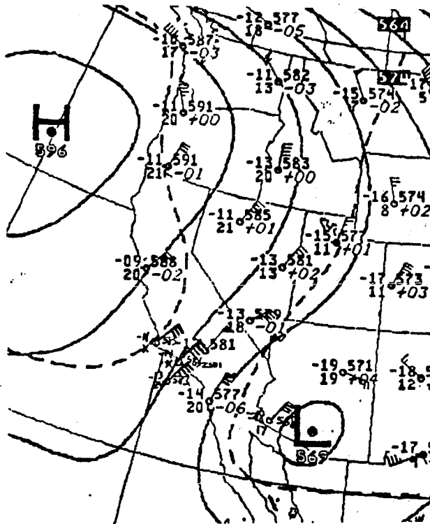
FIGURE 6a. 1200 UTC 27 October 1993 500mb analysis heights/temperature
