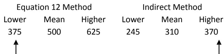
Figure 72. South Fork Thomas Creek Comparison of Results for Peak Flow: The Lower Equation 12 Value for the 5-Year Storm is Essentially the Same as the Higher Indirect Method Value (within 5 cfs).
