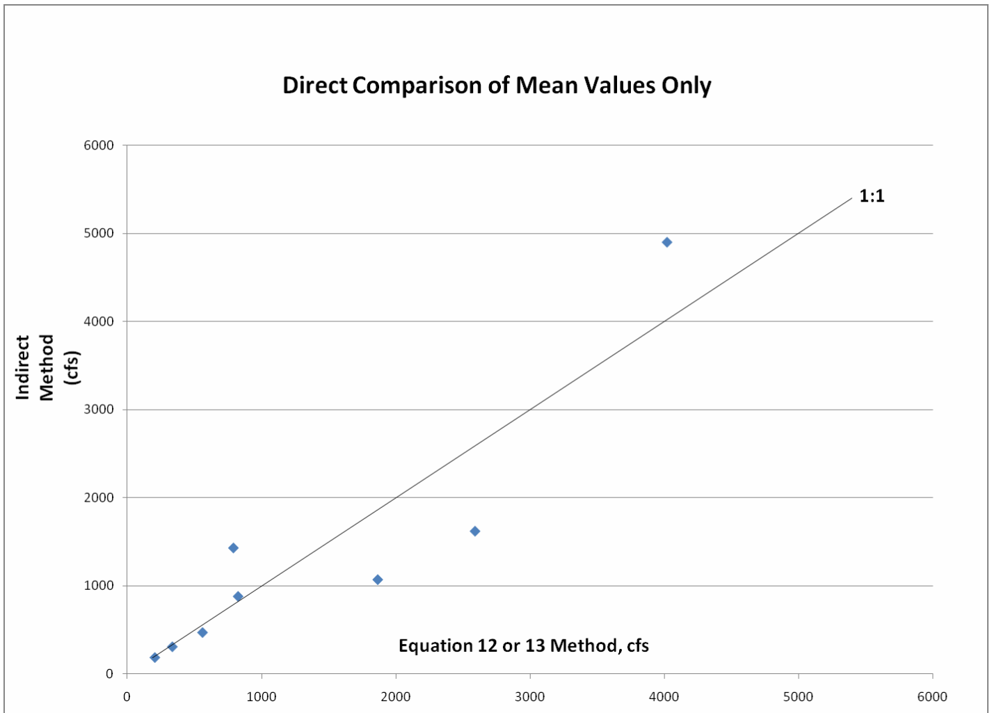
Figure 99. Comparison of Observed and Calculated Peak Flows for Mean Values Only. The four lowest observed peak flow basins (NFT, SFT, ETC, and Cave) line up almost directly with the 1:1 line. The four highest observed peak flow basins (Ash, Hannagan, Old Sawmill, and Miller) are likely outliers either because the return interval was different than that used or because of the uncertainty associated with the indirect method value.
