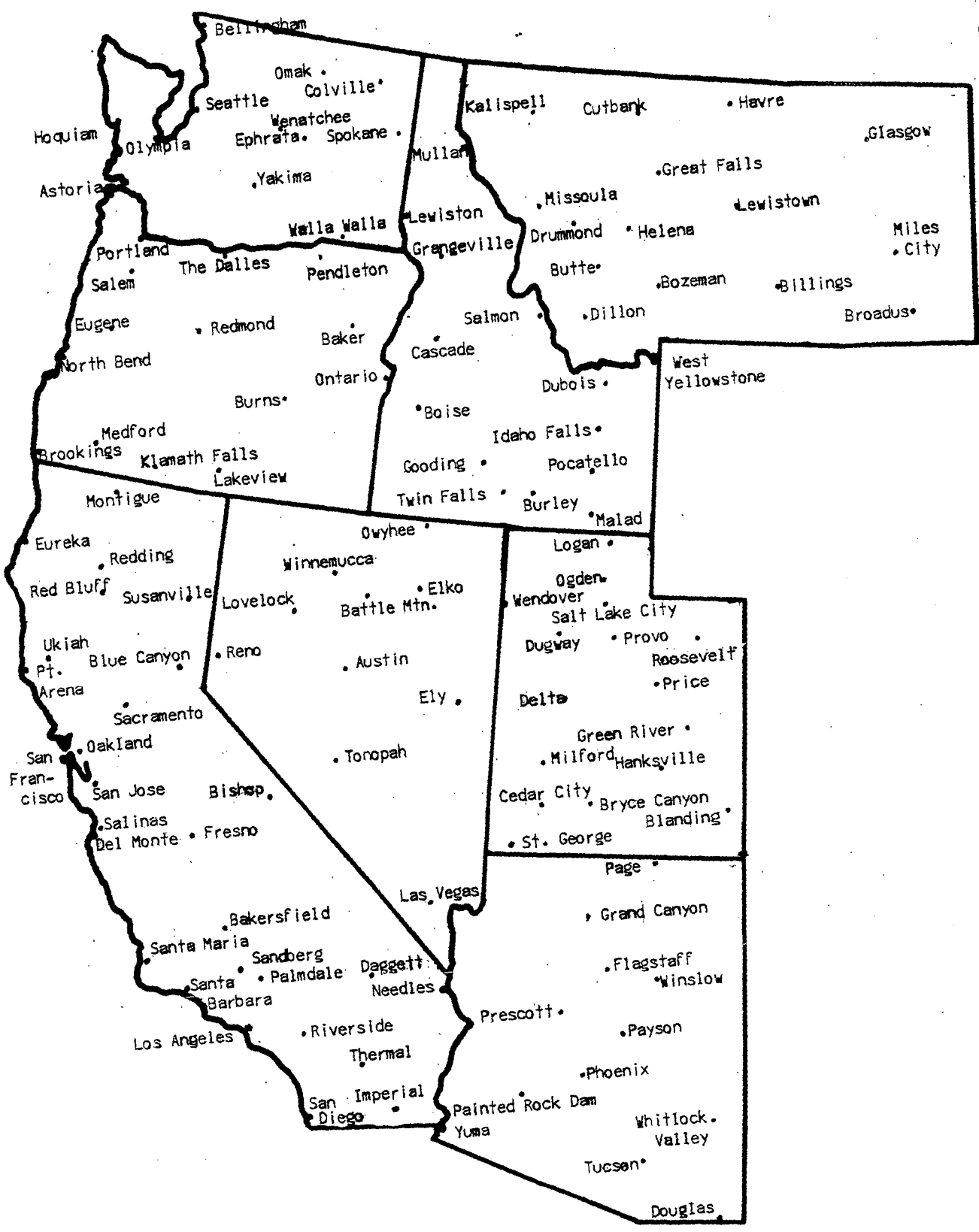
FIGURE 11 DISTRIBUTION OF CLIMATOLOGICAL STATIONS
