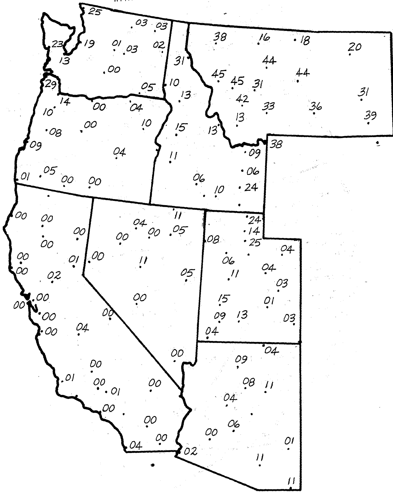
FIGURE 12 PERCENT FREQUENCY OF PRECIPITATION OCCURRENCE WITH 500-MB WINTER TYPE 8
