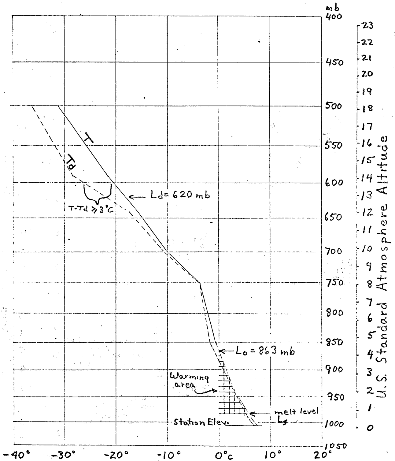
Fig.2 Oakland sounding 2-6-69 1200Z
