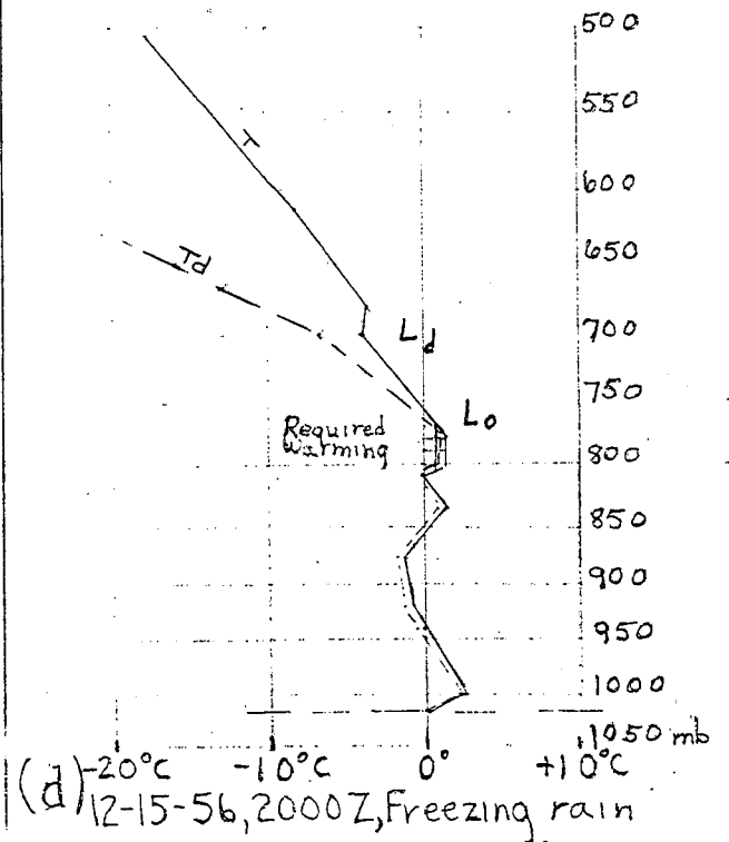
Figure 3. Boston Soundings (after Wagner)
