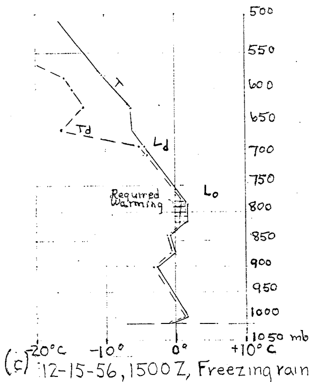
Figure 3. Boston Soundings (after Wagner)
