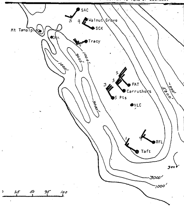
FIGURE 17C. WINDS 293 M. ABOVE GROUND LEVEL AT 2115 PST AUGUST 2, 1971.
