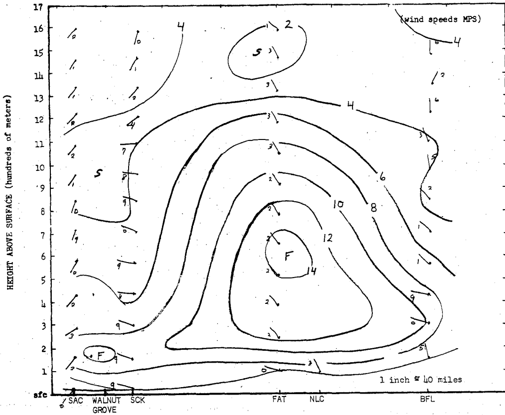
FIGURE 11E. LONGITUDINAL SECTION, SACRAMENTO-BAKERSFIELD, FOR 2115 PST AUGUST 2, 1971.
