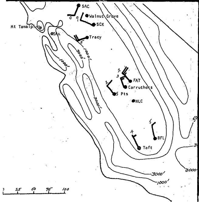
FIGURE 17G. WINDS 829 M. ABOVE GROUND LEVEL AT 2115 PST AUGUST 2, 1971.
