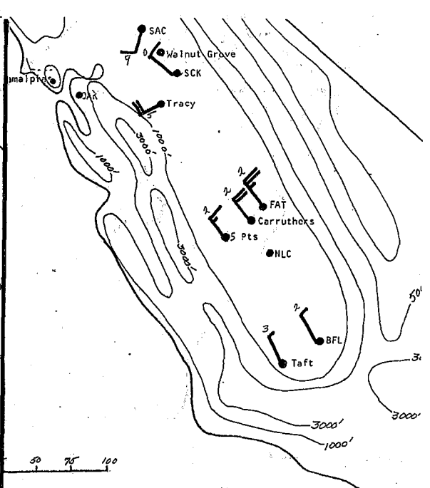
FIGURE 17F. WINDS 701 M. ABOVE GROUND LEVEL AT 2115 PST AUGUST 2, 1971.
