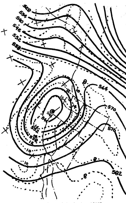
Figure 33a. Initial Analysis, 1200Z, Thursday, April 25, 1974.
