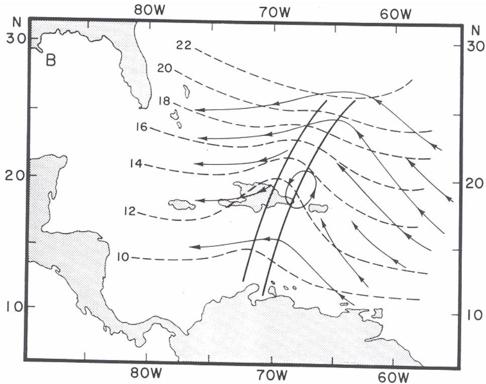
Figure 4. Characteristic pattern in the low-level pressure and wind field for tropical waves.
