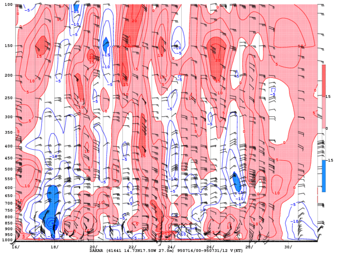
Figure 5. An example from mid-July 1995, showing a trio of waves emerging off the coast of west Africa.
