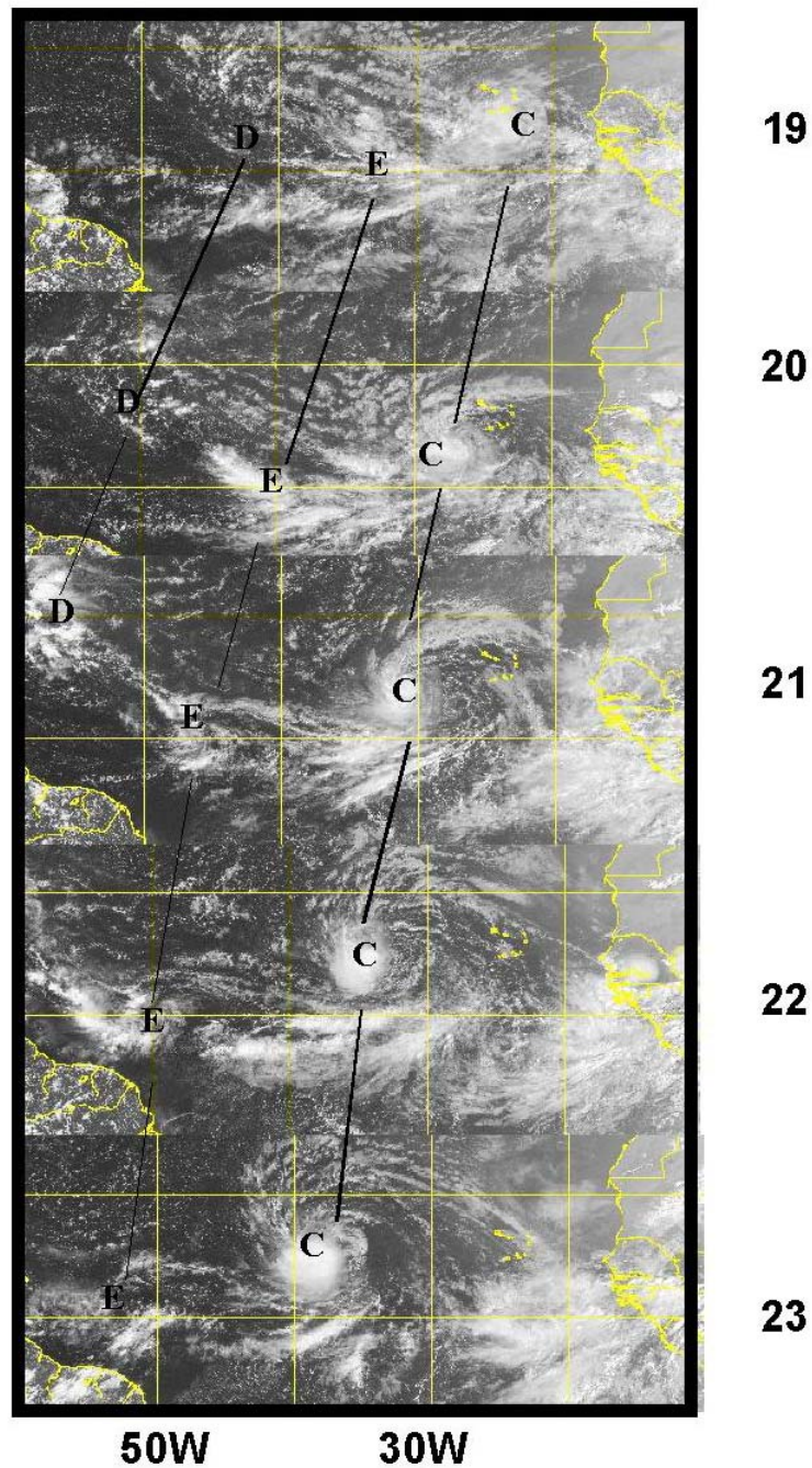
Figure 11. Satellite imagery-based Hovmoeller diagrams showing day-to-day shifts in the position of tropical waves in the deep tropics from August 1999, showing the tropical waves associated with the formation of Cindy, Dennis, and Emily.
