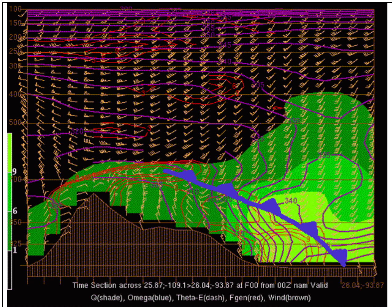
Figure 6. An example of a cross section which can be generated on AWIPS at the various analysts centers for use in real-time surface analyses. The position of the front is shown.
