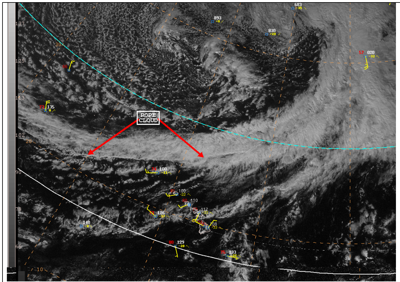
Figure 10. GOES visible imagery depicting a frontal rope over the Central Pacific Ocean.
