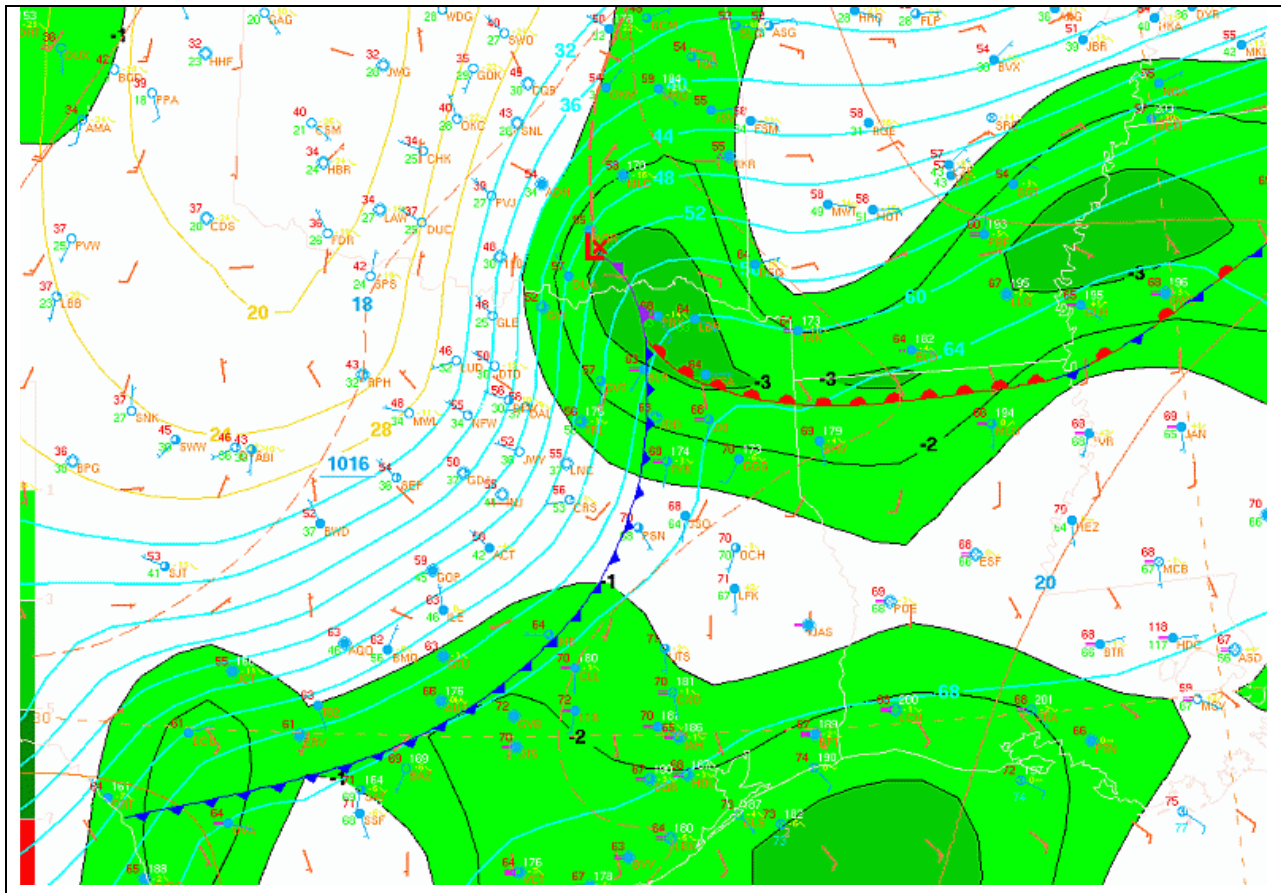
Figure 14. An example of the moisture convergence field, with surface observations included.
