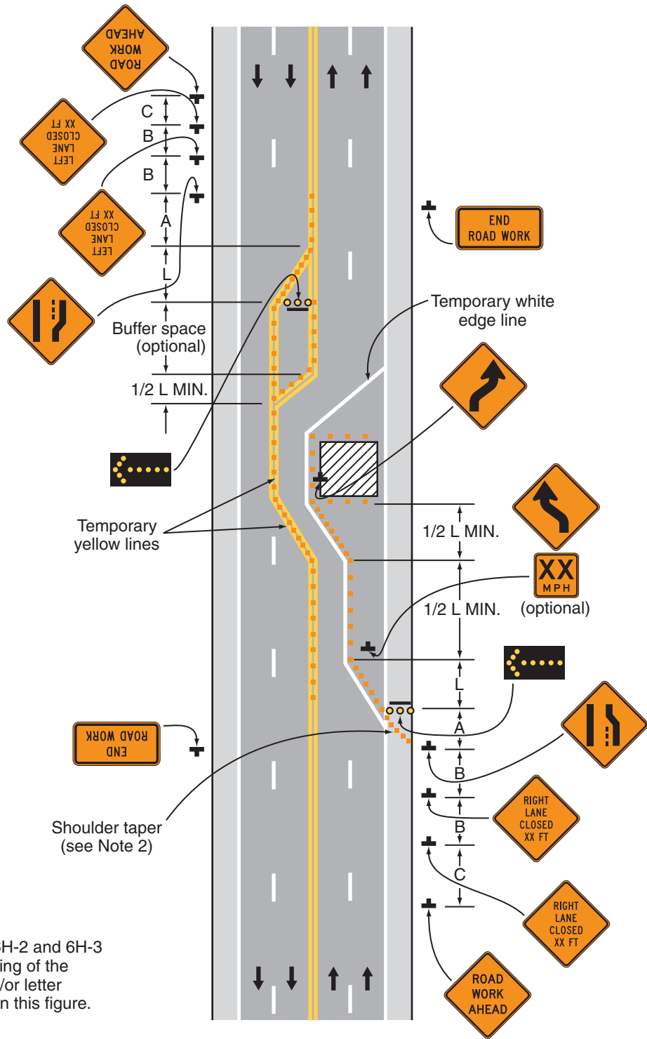
Typical Application 32
