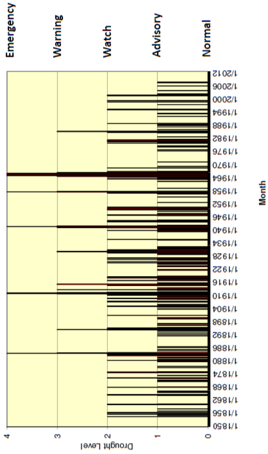
Statewide Drought Levels using SPI Thresholds 1850 to 2012 (Actual Drought Levels 2001 to 2012)
