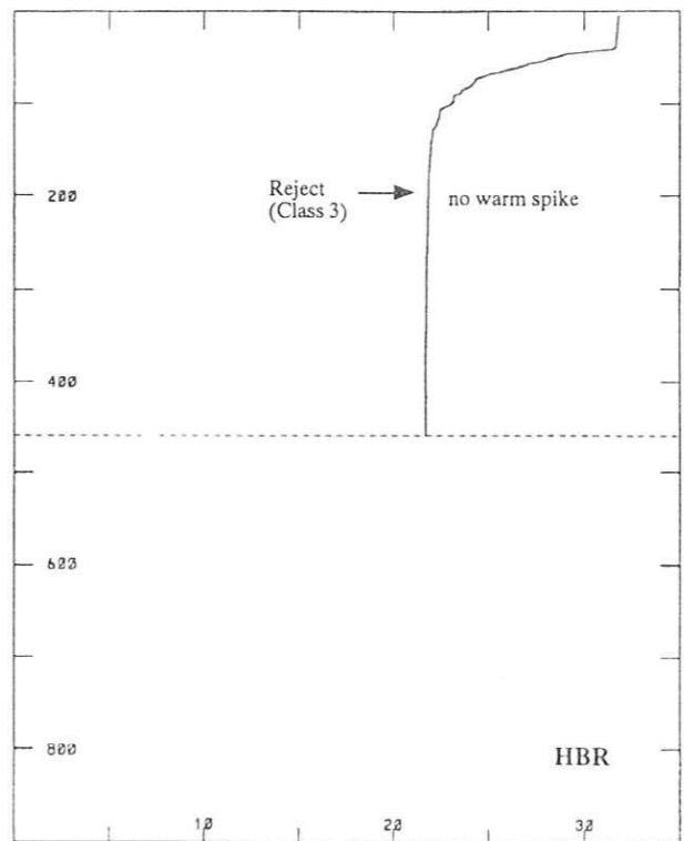
Figure 3.1R Hit Bottom Reject (HBR)
