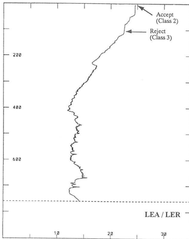
Figure 5.4A Leakage Accept/Reject (LEA/LER)
