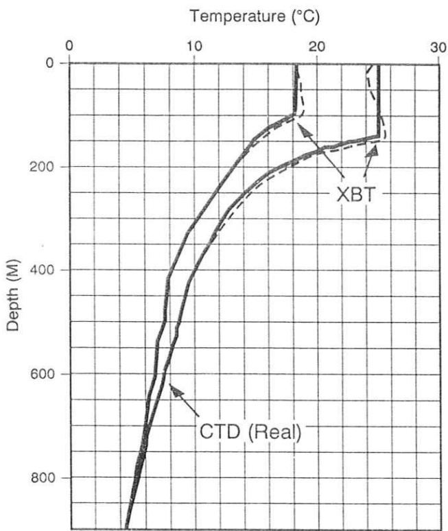
Figure 2.6 Bathymetry Systems Bowing Problem or Bowed Mixed Layer
