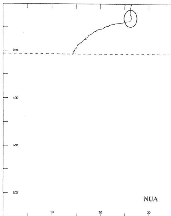
Figure 4.2.2 Inversion in Mixed Layer Confirmed "Nub" (NUA)
