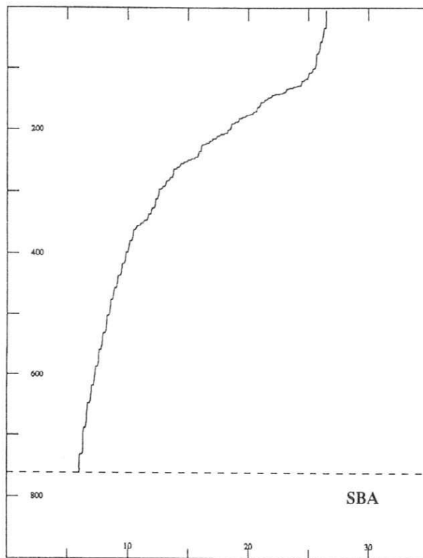
Figure 2.7A Sticking Bit Problem Accept (SBA)
