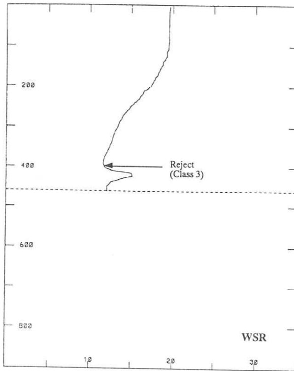
Figure 4.5.1 Wire Stretch Reject (WSR)
