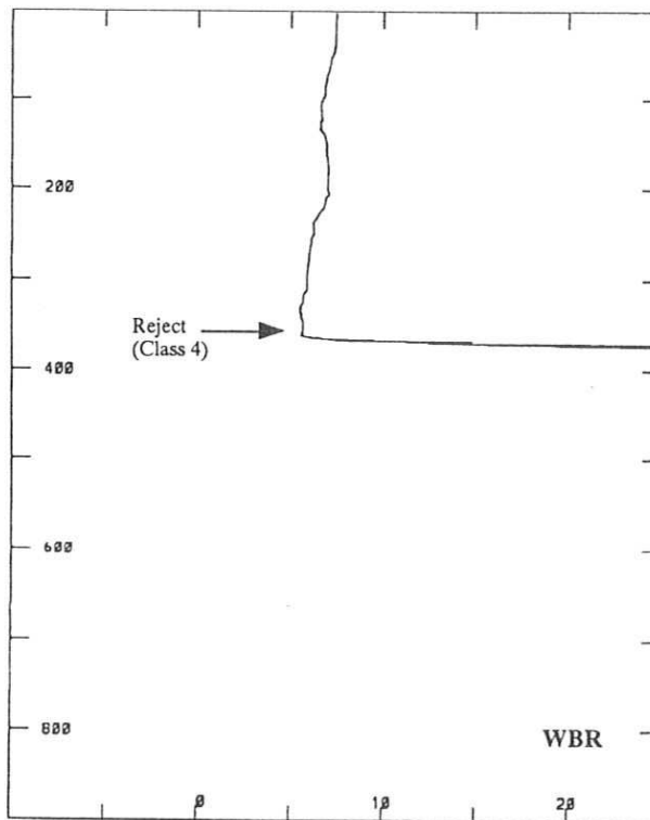
Figure 3.2R.2 Wire Break Reject From Probe Spool (WBR)
