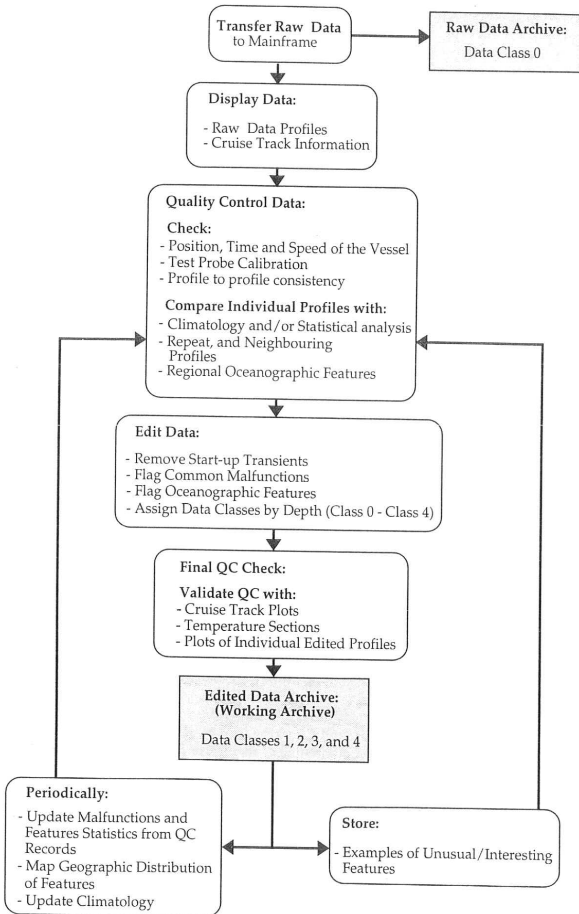
Figure 2 CSIRO XBT Quality Control Process
