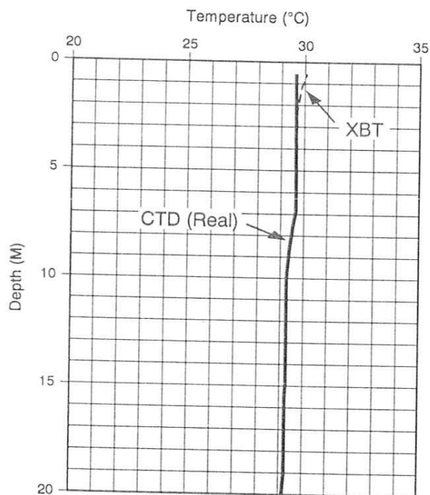
Figure 2.1 Surface Spike Start up Transient Problem (CS)
