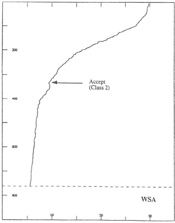
Figure 4.4.2 Wire Stretch Accept (WSA)
