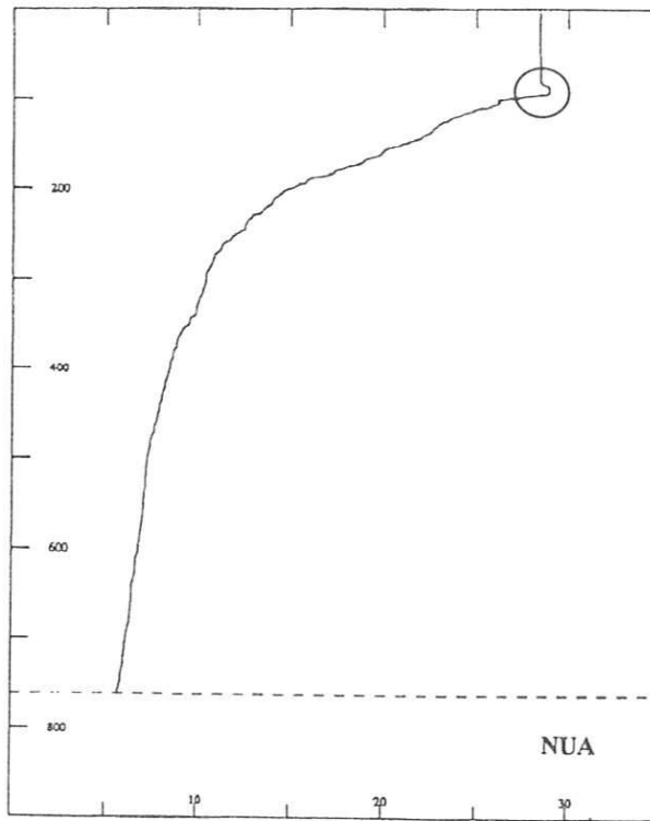
Figure 4.2.1 Inversion in Mixed Layer Confirmed "Nub" (NUA)
