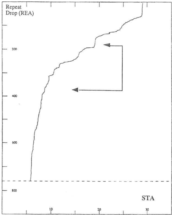
Figure 5.1a Fine Structure (Step-Like) Confirmed (STA)
