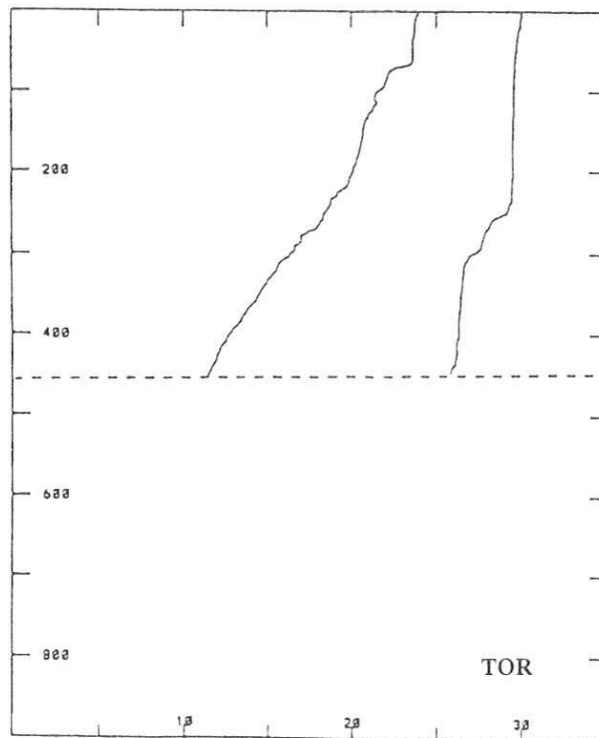
Figure 6.3 Temperature Offset Reject (TOR)
