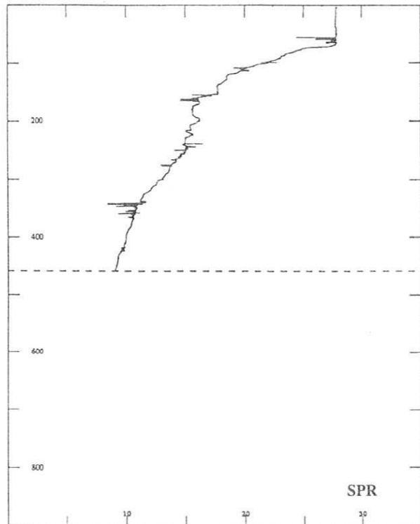
Figure 3.3R Spikes Reject (SPR)
