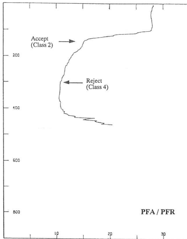
Figure 2.4 PET Fault Accept / Reject (PFA/PFR)
