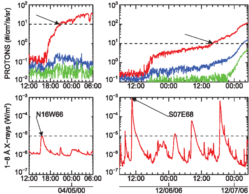
Figure 1. (top) Two SEP events from the primary data set showing the GOES E > 10 MeV (red), E > 50 MeV (blue), and E > 100 MeV (green) proton intensities. The E > 10 MeV thresholds of 10 pfu are indicated by the arrows. (bottom) The associated GOES 1–8 Å solar X-ray flares with peak times indicated by arrows. Time scale is HH:MM in UT. (left) The SEP event of 4 April 2000 associated with an M1 flare at W66° has a rapid increase to the 10 pfu level 5.2 h after the flare peak. (right) The SEP event of 5 December 2006 has a 29.3 h delay to 10 pfu following the peak of the X9 flare at E68°. [from Kahler and Ling, 2015, citation above.]
