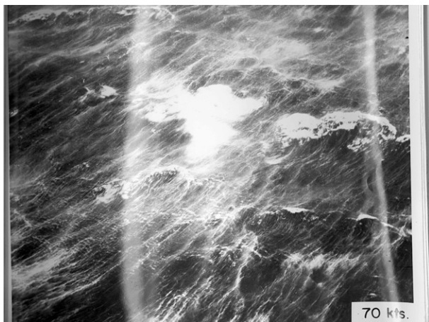
FIG. 1. Photograph of the sea surface in 70-kt winds (from Neumann 1952).
