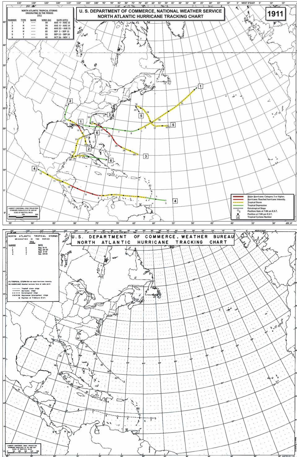
FIG. 2. The (top) revised and (bottom) original Atlantic basin TC track map for 1911, 1912, 1913, 1914, 1915, 1916, 1917, 1918, 1919, and 1920.
