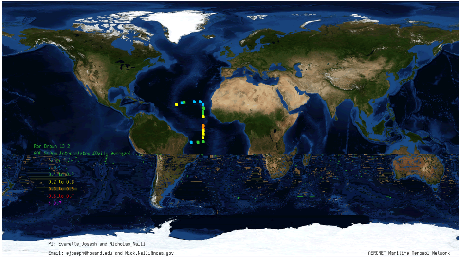
Figure 18 AEROSOL 2013b Microtops sunphotometer solar-spectrum AOD measurements at 0.5 micrometers (GSFC Maritime Aerosol Network processing).
